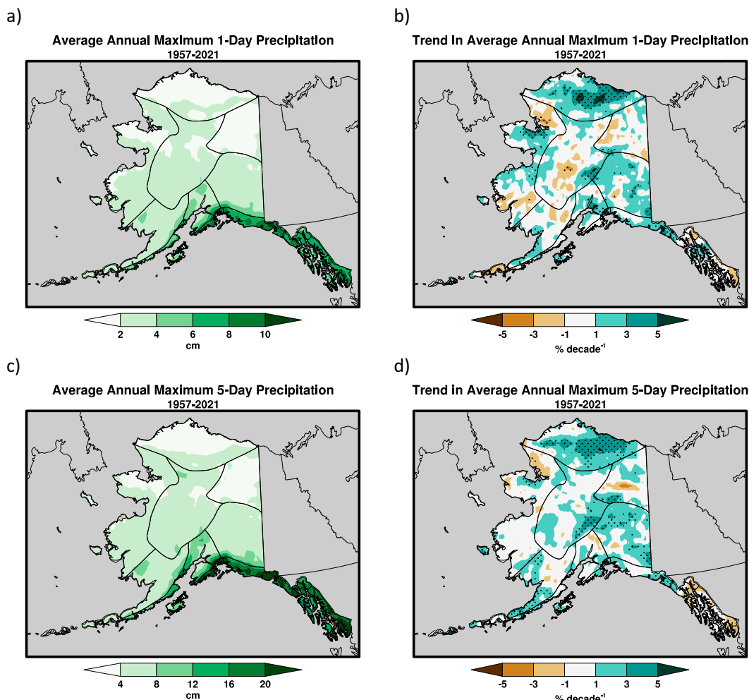
FIG. 8. (left) Mean values (cm) and (right) Theil-Sen trends (% decade -1 ) of annual (a),(b) maximum 1-day precipitation and (c),(d) maximum 5-day precipitation. Significant trends, where p \leq 0.10 , are stippled.
