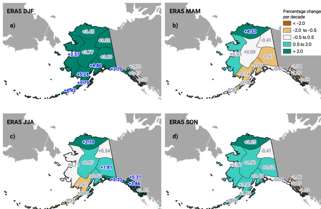
FIG. 7. Seasonal ERA5 precipitation Theil-Sen climate division trends (% decade -1 ), 1957–2021, for (a) winter (DJF), (b) spring (MAM), (c) summer (JJA), and (d) autumn (SON). Blue, bolded values indicate trends that are statistically significant at p \leq 0.10 .
