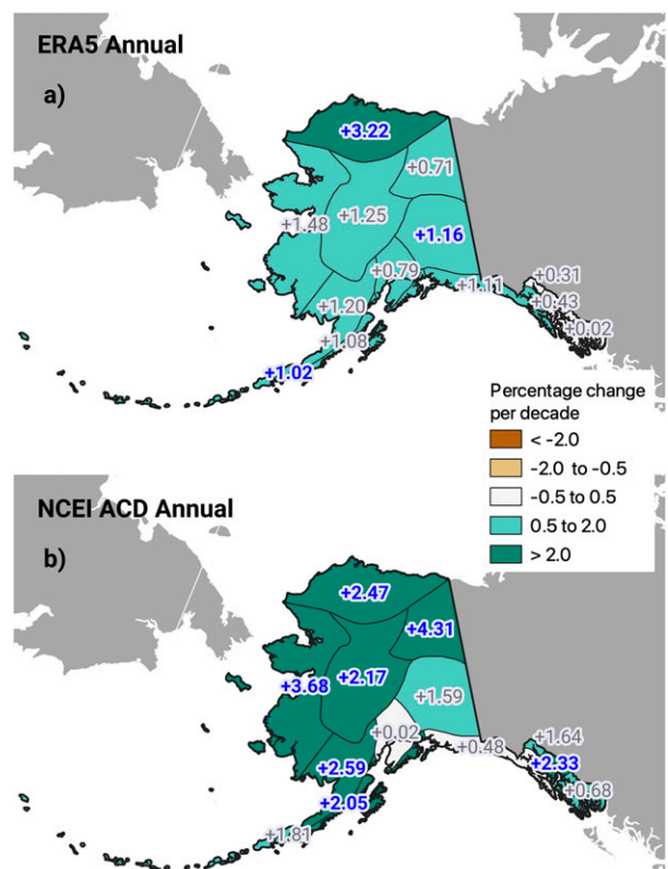
FIG. 6. Annual precipitation Theil–Sen climate division trends (% decade −1 ) for (a) ERA5 and (b) NCEI ACD. Blue, bolded values indicate trends that are statistically significant at p \leq 0.10 .
