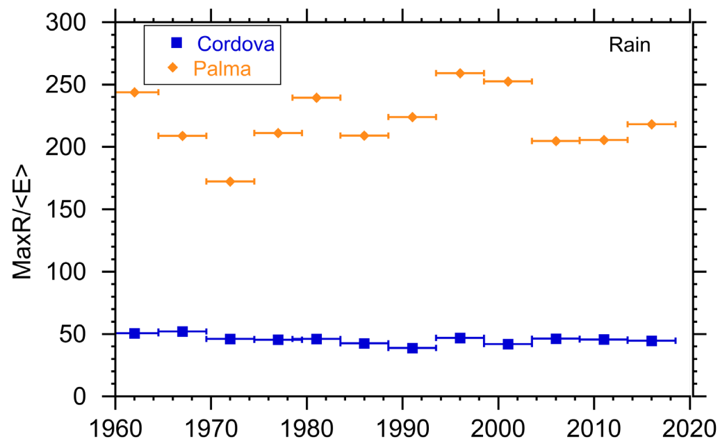
Figure 11. Ratio of the energy storage needed to the average daily energy produced by hydro plants in Cordova and Palma de Mallorca. \text{MaxR}/\langle E \rangle is unitless. Horizontal bars indicate interval over which the parameter was calculated.
