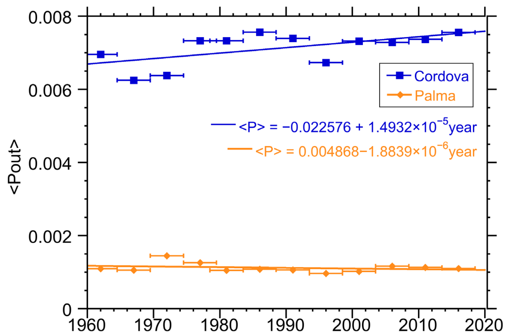
Figure 10. Power production at hydro plants in Cordova and Palma de Mallorca. Power has units of kilowatts. Horizontal bars indicate interval over which the parameter was calculated.
