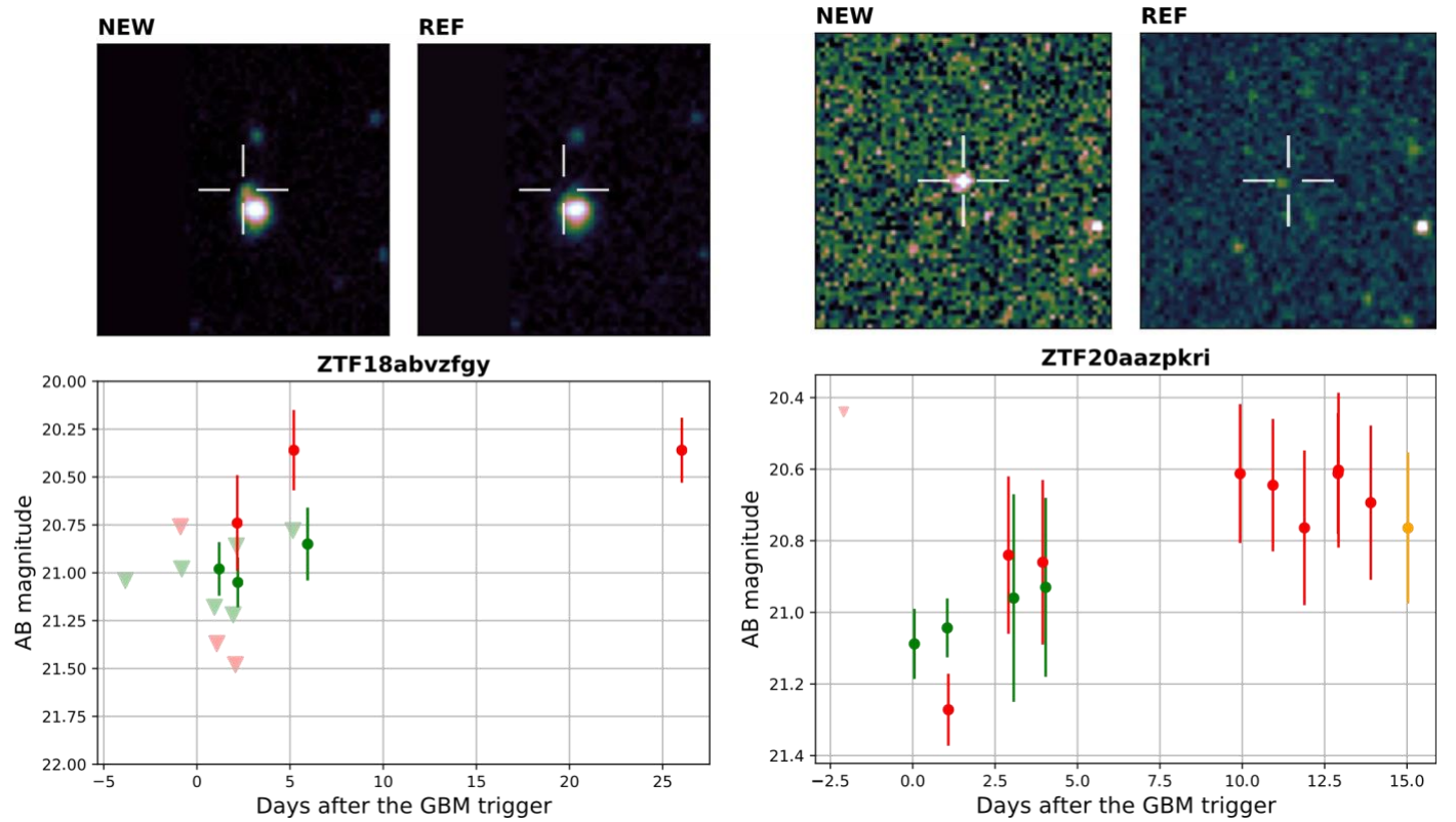
Figure 5. Examples of light curves and cutouts for candidates that passed our filtering criteria. Candidate ZTF18abvzfgy (candidate counterpart to GRB 180913A) in the left panel and ZTF20aazpkri (candidate counterpart to GRB 200514B) in the right panel. The observations in the g and r bands are plotted in green and red colors, respectively. Filled circles represent ZTF detections, while the 5\sigma upper limits are shown as triangles in the light curve. The top half of each panel shows the discovery image on the left and the reference image on the right. In the 0.7 \text{ arcmin}^2 cutouts, north is up and east is to the left. A cross marks the location of the transient. to 200 Mpc, the GW170817 light curve overlaps with the region of five of our searches, suggesting that the combination of depth and rapid coverage of the regions could allow us to detect a GW170817-like event. The searches that do not overlap with the scaled GW170817 have either fainter median magnitude upper limits ( < 20 \text{ mag} ) or late starting times ( > 1 \text{ day} ).
