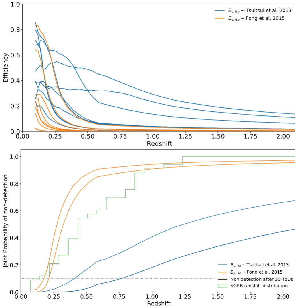
Figure 9. (top) The individual efficiency for each SGRB trigger. The blue curves are based on the E_{iso} derived from the Band model E_p and Equation (1), while the yellow curves are the efficiencies assuming all GRBs have the same E_{iso} as the mean E_{K,iso} from Fong et al. (2015). (bottom) The solid lines represent the joint probability of non-detection using the 9 SGRB triggers with no optical counterparts. We adopt the same color coding as in the top plot, meaning blue for the E_{iso} as a function of E_p and yellow for E_{iso} as the mean E_{K,iso} from Fong et al. 2015. The dashed line represent the joint probability of non-detection after 30 ToOs, assuming an efficiency equal to the median efficiency of the ToOs presented. We show the cumulative redshift distribution for SGRBs as a green line. The gray dotted line shows the CL = 0.9 level, at which the joint probability of non-detection is 1 - \text{CL} = 0.1 .
