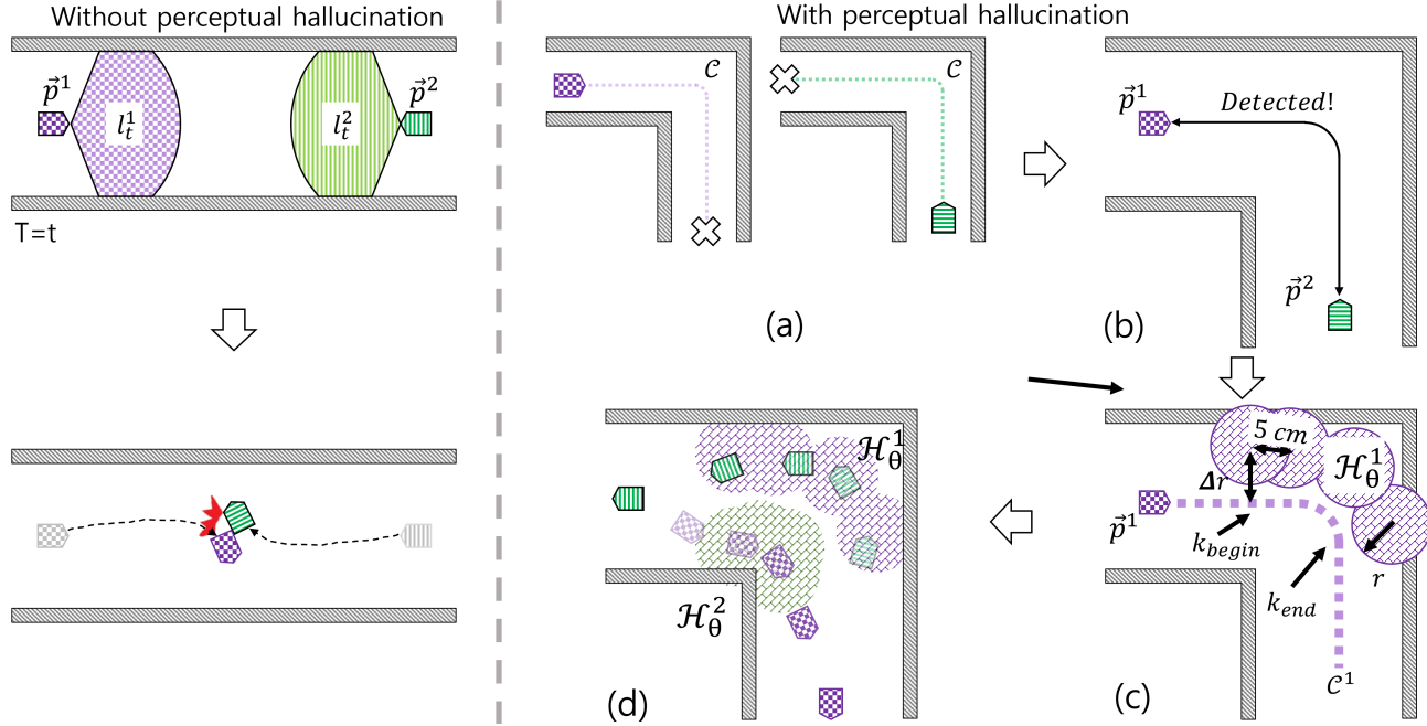
Fig. 1: Overview of the proposed Perceptual Hallucination for Hallway Passing approach. (Left) multi-robot hallway passing scenario with an existing navigation system, and (right) how PHHP improves the navigation system with hallucinated sensor readings. PHHP deployment proceeds as follows: (a) two robots try to pass each other in the hallway; (b) one robot detects the other and initiates the hallucination process; (c) the trained PHHP system generates a hallucinated field \mathcal{H}_\theta in the global coordinate system based on the global plan (d) each robot uses its corresponding hallucinated scan l_{\theta} and its existing navigation system to handle the rest of the scenario. Note that the hallucination function, h(l, \mathcal{H}) , computes the depth value of hallucinated readings by taking the minimum value between the real and virtual scans.
