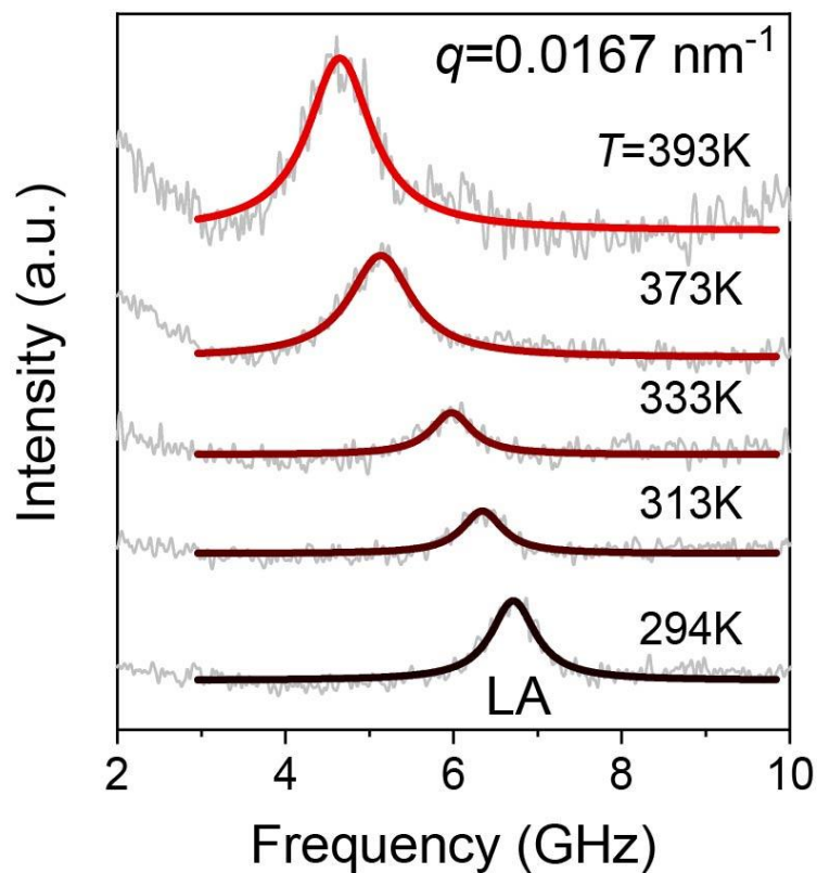
Supplementary Figure 10. Temperature-dependent polarized BLS spectra for the polydomain LCE. At a given q=0.0167 \text{ nm}^{-1} , the single peak is assigned to longitudinal acoustic (LA) phonon. The BLS spectra is represented by Lorentzian shapes (colored lines).
