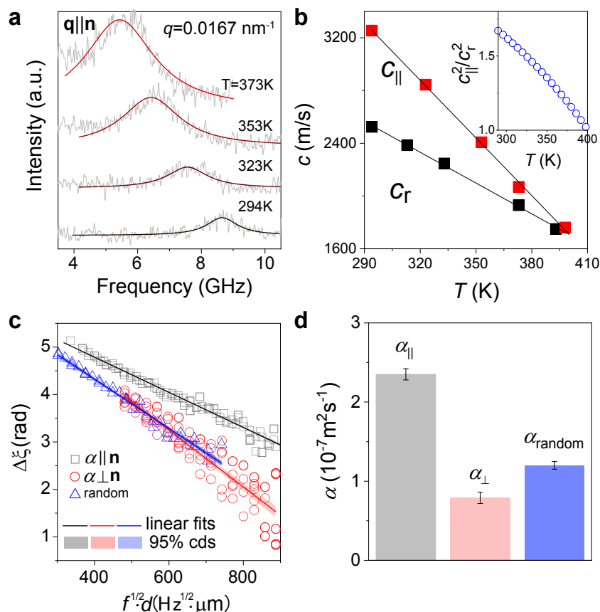
Fig. 4 | Temperature-dependent elasticity and anisotropic thermal diffusivity. a Evolution of polarized BLS spectra with the temperature at a given q parallel to n . b The temperature-dependence of c_{\parallel} in monodomain LCE and c_r in polydomain LCE along with their ratio shown in the inset. The solid lines denote linear representation of the temperature-dependent sound velocities. c The phase delay \Delta\xi of the heat waves traversing the LCE films with a thickness d as a function of f^{1/2}d , where f
