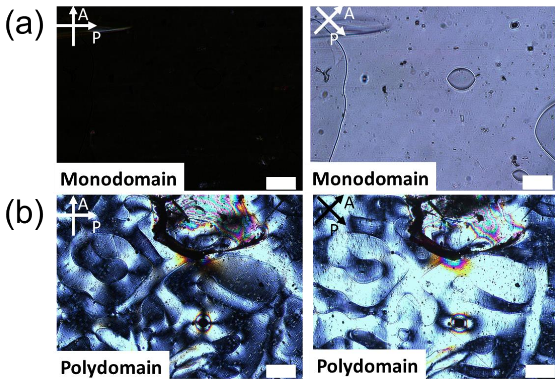
Supplementary Figure 1. Polarized optical microscopy images. (a) monodomain and (b) polydomain LCE films. In the right panel of (a) and (b), the polarizer (P) and analyzer (A) are rotated by 45°. The arrows indicate the polarization of the polarizer and analyzer. (Scale bars: 200 \mu\text{m} )
