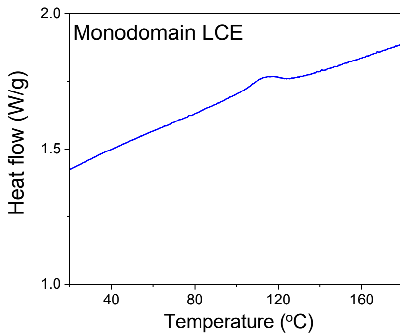
Supplementary Figure 11. Differential scanning calorimetry (DSC) curve for monodomain LCE. The DSC curve, obtained at a heating rate of 10 °C/min, shows the nematic-isotropic transition temperature at T = \sim 390 K.
