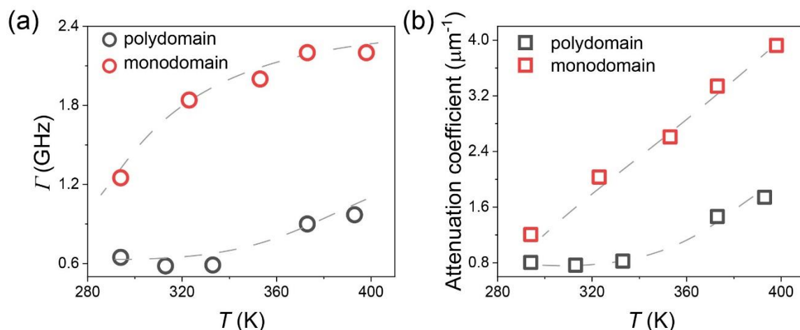
Supplementary Figure 12. Temperature-dependent viscosity. (a) Linewidth and (b) attenuation coefficient \mu(=\pi\Gamma/c) of Q-L and LA phonon in Fig. 4b as a function of temperature. The dashed lines are used to guide the eyes.
