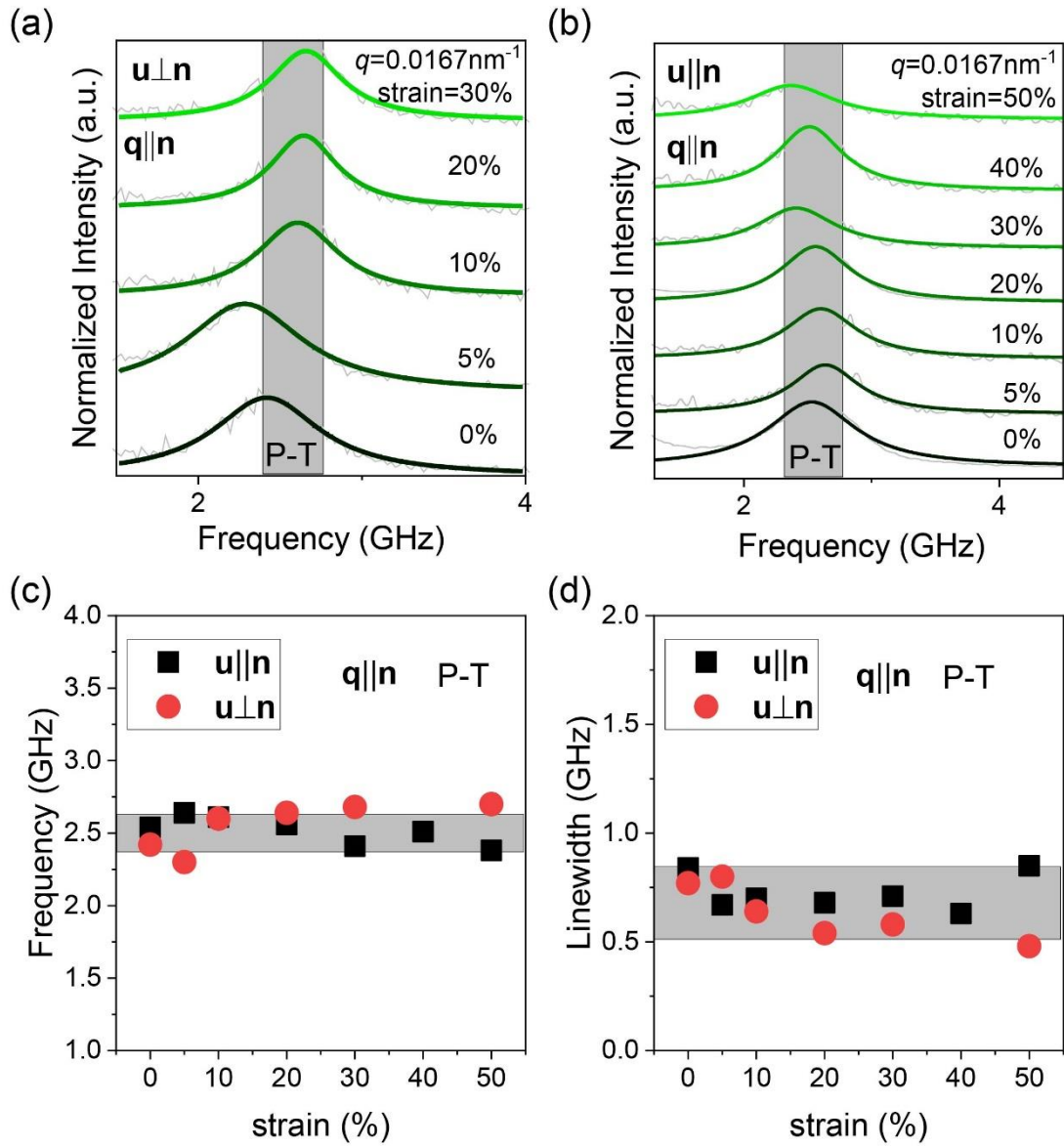
Supplementary Figure 8. Evolution of pure transverse mode on strain for monodomain LCE. At a given q=0.0167\text{nm}^{-1} which is parallel to the director \mathbf{n} , strain-dependent depolarized (VH) BLS spectra under uniaxial stretching being (a) normal and (b) parallel to the director \mathbf{n} , respectively. The single peak is assigned to pure transverse (P-T) phonon. The corresponding frequency and linewidth of P-T modes is shown in (c) and (d), respectively. The BLS spectra is represented by Lorentzian shapes (colored lines). The shaded area denotes the invariant of the physical quantities.
