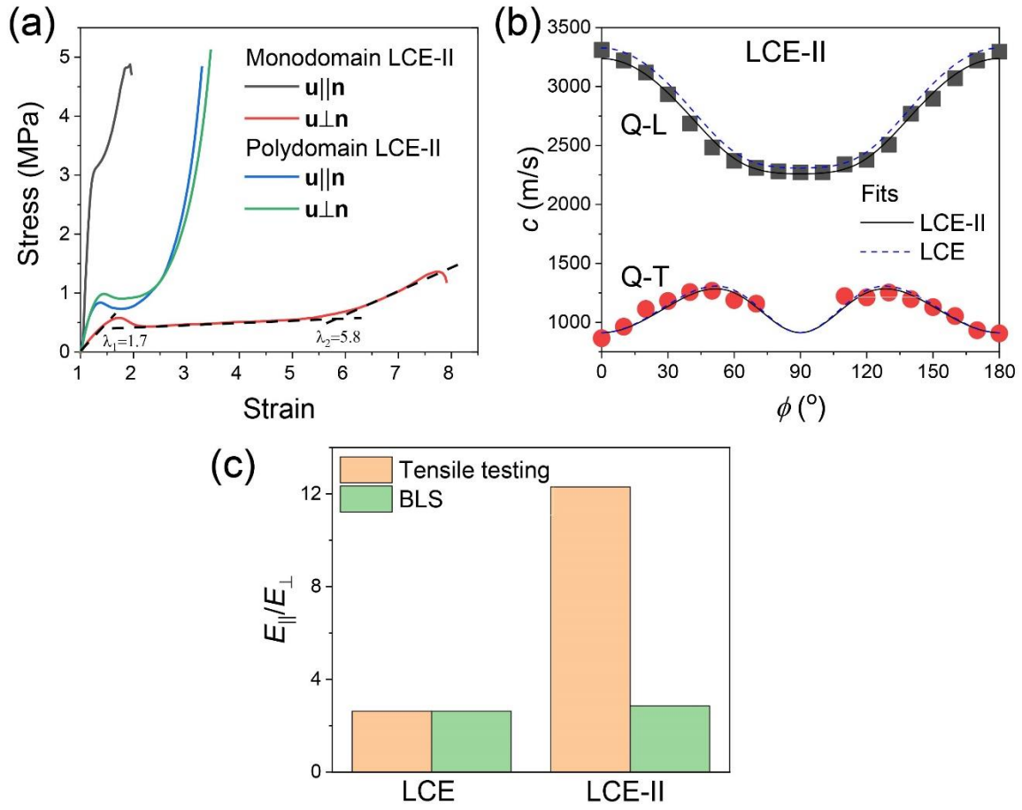
Supplementary Figure 7. Elastic anisotropy of LCE-II film measured by tensile testing and BLS. (a) Strain-stress curves of LCE-II films in monodomain and polydomain states with extension being parallel and perpendicular to the director \mathbf{n} , respectively. The \lambda_1 and \lambda_2 are estimated according to literature 2,3 from intersection of dash lines representing the low-strain linear, soft-plateau, and high-strain linear regimes, respectively. (b) Sound velocities of Q-L and Q-T modes vs. orientation angle \phi of monodomain LCE-II film. The black solid lines and blue dashed lines are fits for LCE-II and LCE respectively. (c) Comparison of Young's modulus anisotropy, E_{\parallel}/E_{\perp} , obtained from tensile testing and BLS respectively.
