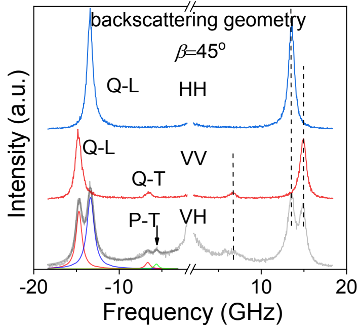
Supplementary Figure 5. VV, HH, and VH BLS spectra obtained at the backscattering geometry for monodomain LCE film. At incident angle \beta=45^\circ , the Q-L and Q-T modes in VH spectra corresponds to that in the VV and HH spectra due to the birefringence. The lowest-frequency peak in VH spectra but absent in the polarized spectra can be assigned to pure transverse (P-T) mode. The VH spectra are represented by the Lorentzian shapes (thick grey line) with four individual peaks (colored lines). The dashed lines are guide to the eye. The two P-T data at high orientation angle \phi 's (Fig. 2c) allow the determination of C_{66} according to \rho \left(\frac{2\pi}{q}\right)^2 f_{P-T}^2 = \sin^2 \phi C_{66} + \cos^2 \phi C_{44} (solid line in Fig. 2c). f_{P-T} = f_{Q-T} is valid when \phi = 0^\circ . Other four independent elastic constants ( C_{11} , C_{33} , C_{13} and C_{44} ) are mainly determined by f_{Q-L}(\phi) and f_{Q-T}(\phi) .
