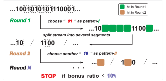
Fig. 4: The illustration of multiple rounds mining.
