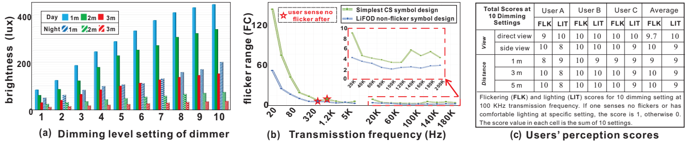
Fig. 13: Evaluation of fine-grained dimming and non-flicker performance.
