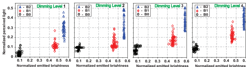
Fig. 9: Grayscale diagram of B0, B1, B2 on four incremental dimming levels.
