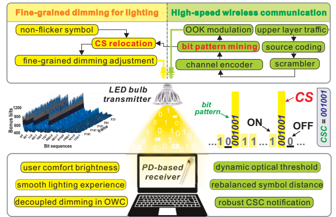
Fig. 2: System architecture and workflow of LiFOD.
