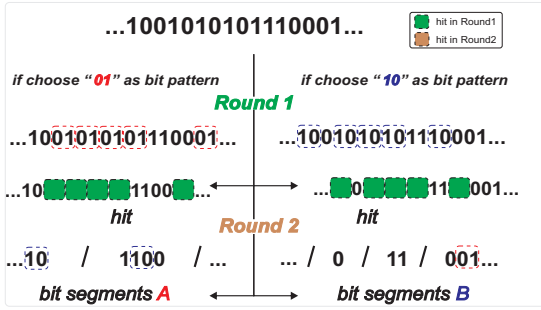
Fig. 3: Bit pattern candidates change in next round.
