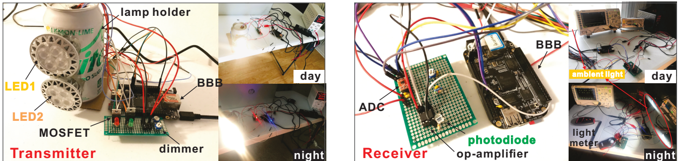
Fig. 12: LiFOD prototype: transmitter, receiver and experiment scenarios in day and night.
