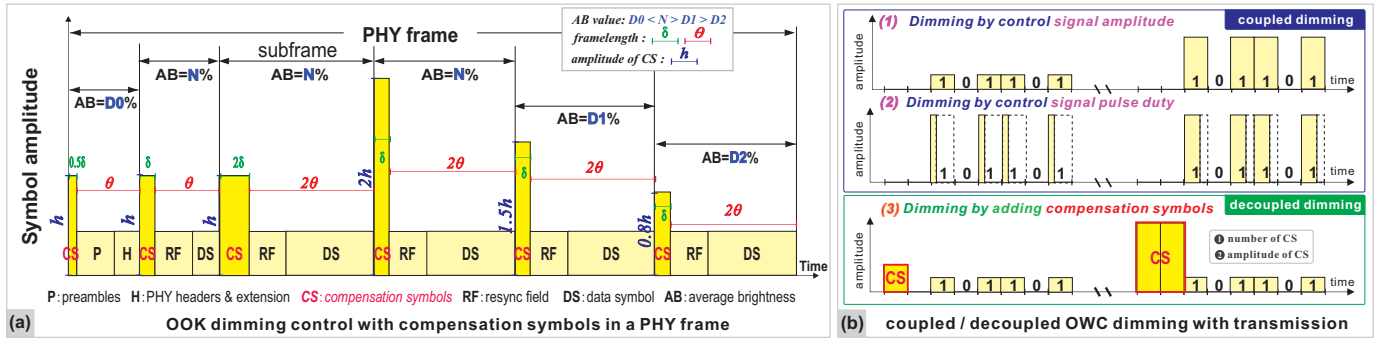
Fig. 1: (a) Adjust CS frame with varied symbol amplitude and frame length for OOK dimming, redesigned from IEEE standard [17]. (b) CS dimming is decoupled with transmission by adding variable number and amplitude of compensation symbols.
