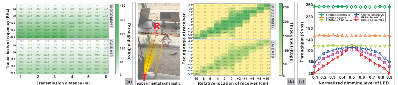
Fig. 14: Throughput performance evaluation of LiFOD. (a) Throughput vs. distance and frequency, (b) Throughput vs. incidence angle and position, and (c) Comparison with state-of-art [25].
