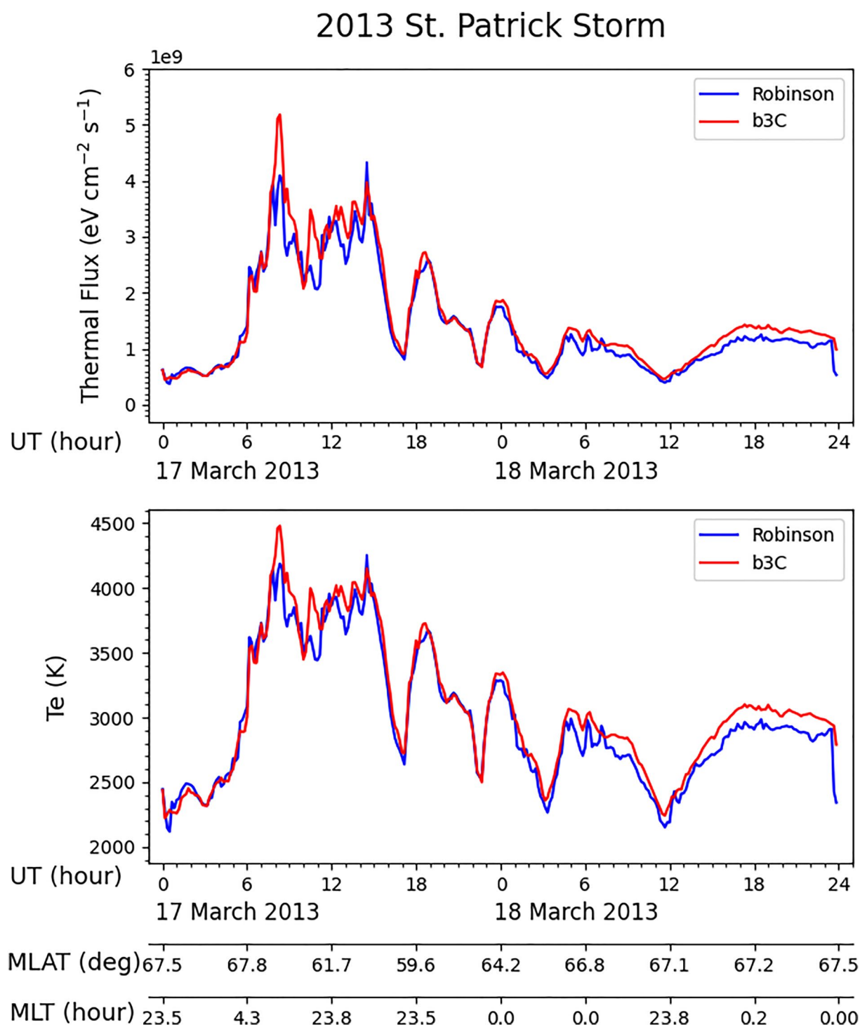
Figure 13. Geomagnetic storm 17 March 2013. RCM-E/STET-driven electron heat fluxes and the corresponding temperature calculation. MLAT and MLT locations are shown in axes below.
