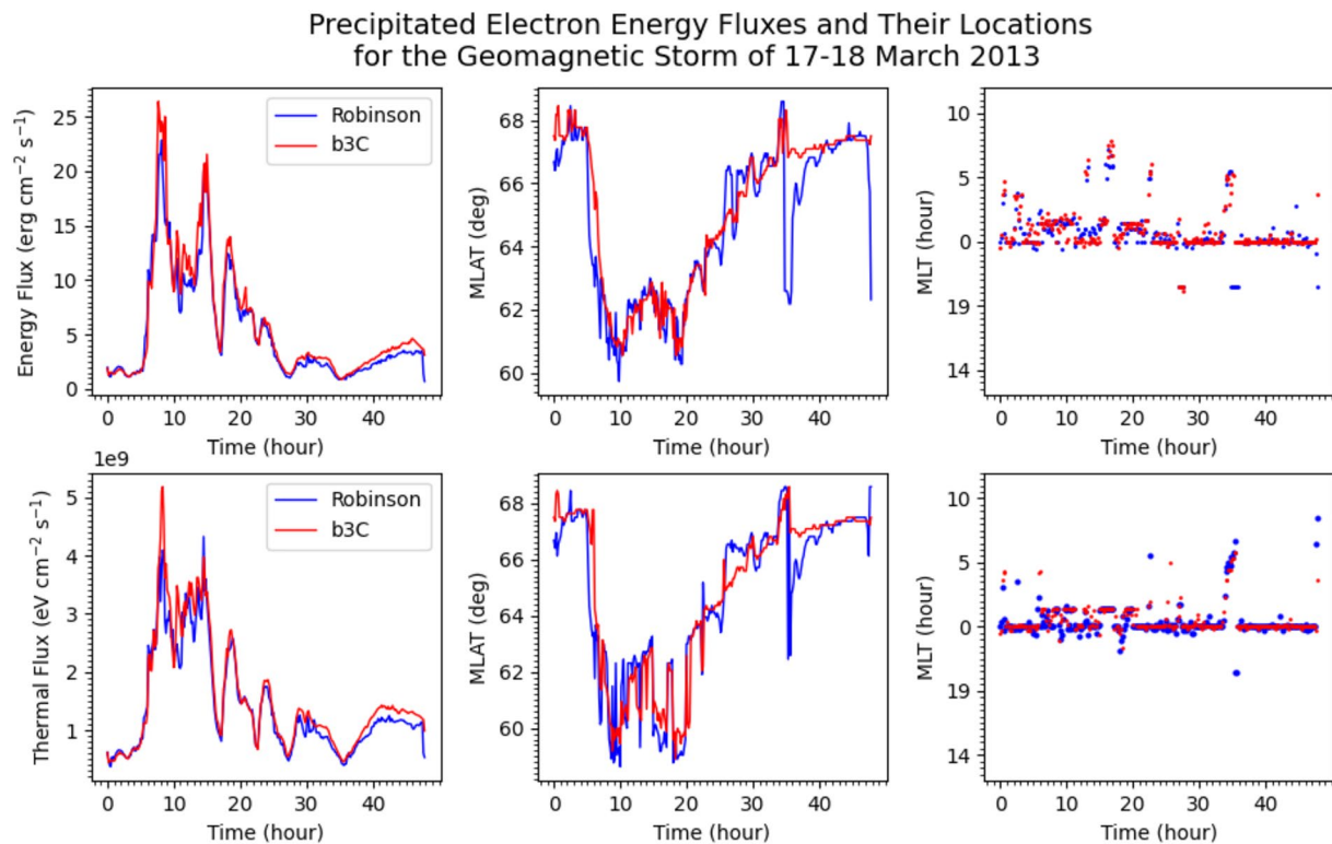
Figure 5. Maximum values of electron precipitation energy and heat fluxes migration over the geomagnetic storm of 17–18 March 2013.
