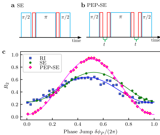
Fig. 3 Improved Ramsey interferometers. a, b Pulse sequences for spin-echo (SE) and pulse-evolve-pulse with spin-echo (PEP-SE) Ramsey interferometers. The red blocks denote the dispersive measurement pulses, and blue bars indicate the microwave pulses. c Interferometer signal measured using: a conventional Ramsey sequence (blue squares), a spin-echo Ramsey sequence (green circles), and a pulse-evolve-pulse with spin-echo sequence (magenta diamonds). All measurements were performed in situ at \bar{\delta} = 63.4 with \bar{t} \approx 7 yielding g \approx 1 .
