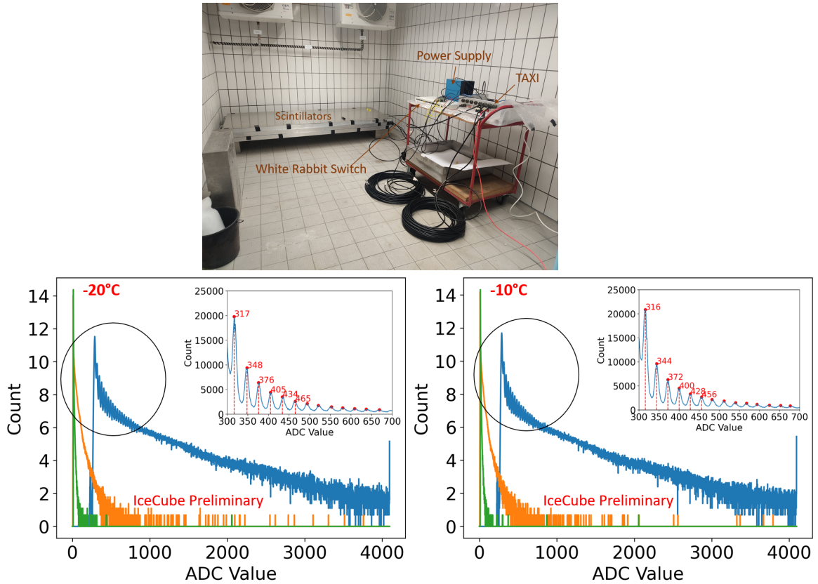
Figure 4: Top: The measurement setup for the low temperature measurements. Bottom: A histogram for the 5 minute measurement, with a focus on the finger spectra, at both temperatures. The blue, orange, and green curves correspond to high-, medium- and low-gain respectively.
