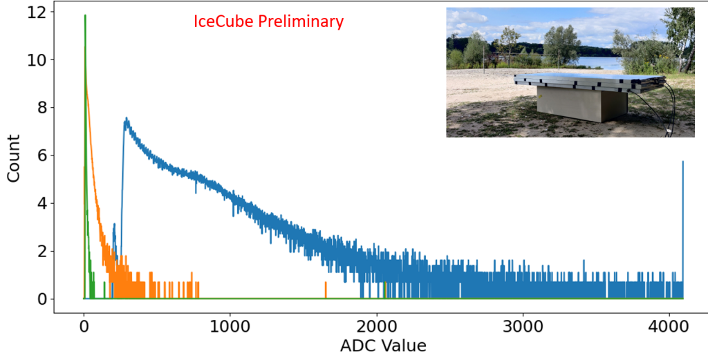
Figure 5: A histogram for the 5 minute measurement for all gains.
