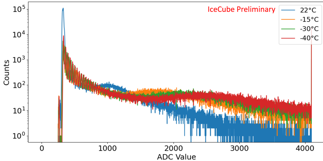
Figure 6: The multi-plot contains high-gain channel histograms for measurements performed at varied temperatures for the same panel.
