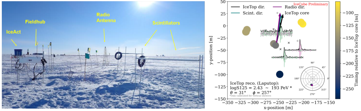
Figure 2: Left: The prototype station currently at the South Pole. Right: An air shower event observed by all three detectors, namely, scintillators, radio and IceTop [9]. The large colored circles signify the scintillator locations and the \times marks the radio detectors.
