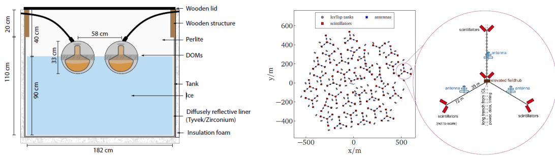
Figure 1: Left: Schematic of an IceTop Cherenkov tank. Each tank consists of two PMT detectors suspended in ice. Right: The footprint of the proposed surface enhancement. A zoom-in of one of the stations is also included to show the positioning of each component [5].
