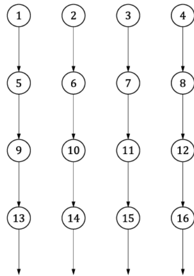
FIG. 12. Graph structure of the auxiliary Hamiltonian H_{\text{aux}} .
