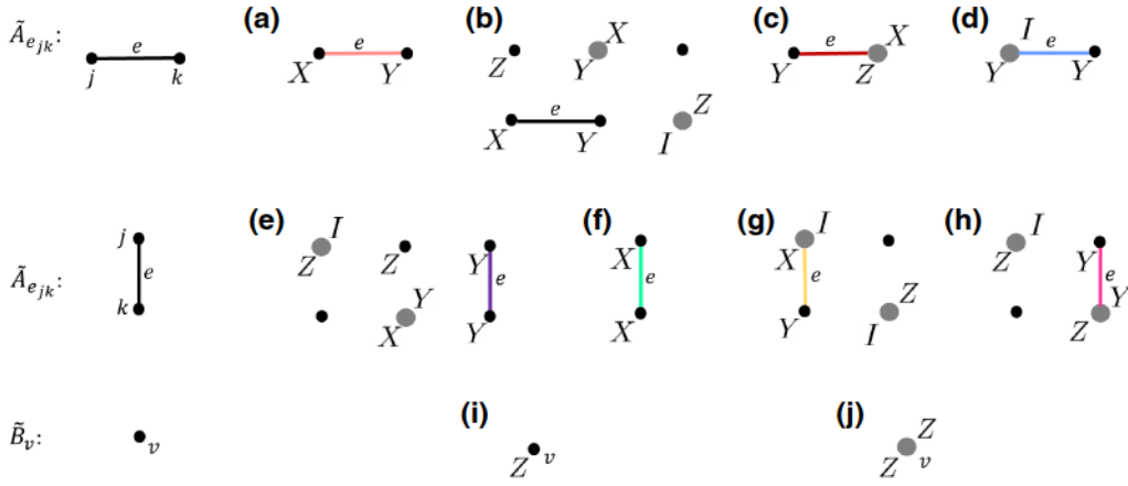
FIG. 26. The hopping term \tilde{A}_{e_{jk}} and the parity term \tilde{B}_v in the bosonic Hilbert space. The definitions of \tilde{A}_{e_{jk}} and \tilde{B}_v depend on the colors of edges and vertices. (a)–(d) Four kinds of horizontal hopping terms; (e)–(h) four kinds of vertical hopping terms; (i), (j) parity terms on black and gray vertices.
