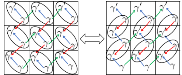
FIG. 6. The r = 1.5 construction is the same as the compact fermion-to-qubit mapping [9] after the re-pairing of Majorana fermions above. Each circle represents a complex fermion formed by the two Majorana fermions. The underlying arrows specify the order to form a fermion. The arrows form a Kasteleyn orientation, ensuring that the fermion parity after re-pairing is well defined [40–42].
