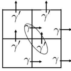
FIG. 14. To match our exact bosonization to the Verstraete-Cirac mapping, we shift our Majorana modes on each face in the following way: (1) shift \gamma'_f upward and let it be \gamma on the new face; (2) shift \gamma_f rightward and let it be \gamma' on the new face.
