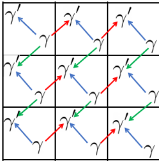
FIG. 18. The embedding of the honeycomb lattice into the square lattice. The red, blue, and green links correspond to the x , y , and z types in Kitaev's honeycomb model.
