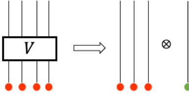
FIG. 1. We disentangle the green qubit from others by a local unitary transformation V and then remove this part. This is called a generalized local unitary circuit.
