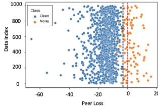
Fig. 1. Peer loss value distribution for random selected 1,000 data instances in CIFAR-10 under symmetric noise (NR = 0.1). x -axis corresponds to peer loss score, and y -axis corresponds to each data instance.
