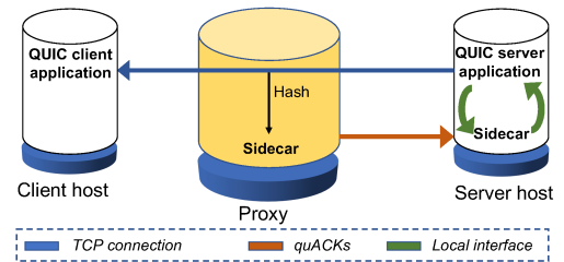
Figure 3: Sidecar ACK reduction.
