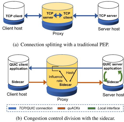
Figure 1: Existing PEPs vs. the proposed sidecar. The transport connection is not interrupted in case (b).
