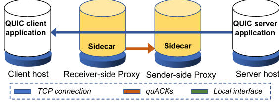
Figure 4: In-network retransmission with the sidecar.
