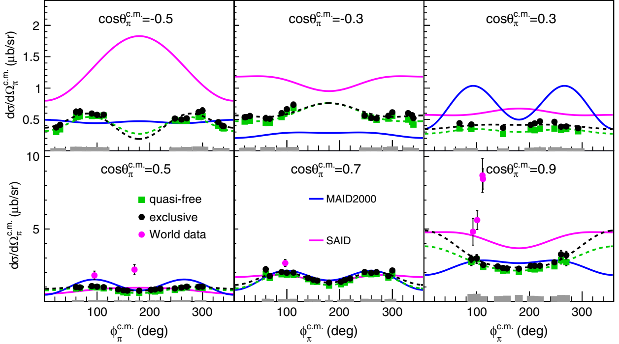
FIG. 27. Full exclusive (black points) and quasifree (green squares) cross sections in \mu\text{b/sr} are presented for W = 1.6625 GeV and Q^2 = 0.5 GeV 2 . The \phi_\pi^{\text{c.m.}} -dependent cross sections are shown in each \cos \theta_\pi^{\text{c.m.}} bin (the bins with reasonable statistics are shown) and the color-matched dashed lines represent the fits to the cross sections by the function a + b \cos 2\phi_\pi^{\text{c.m.}} + c \cos \phi_\pi^{\text{c.m.}} . The magenta and blue solid lines show the SAID [63,64] and MAID2000 [57] model predictions, respectively. The magenta points show the previous available world data [44–46]. The gray bars at the bottom of each subplot quantify the systematic uncertainties of each cross section point and the statistical uncertainties are typically smaller than the data point markers.
