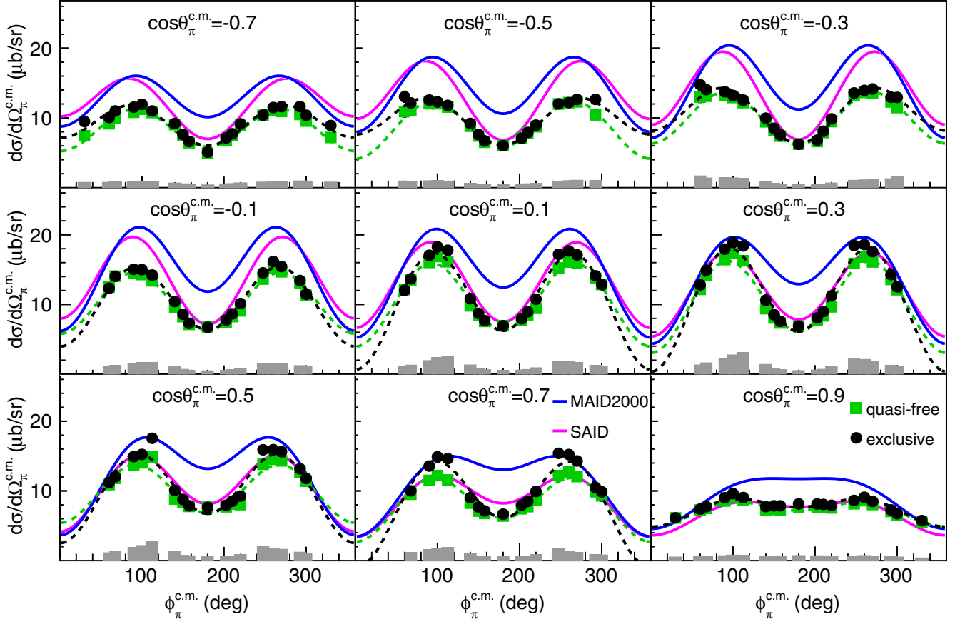
FIG. 25. Fully exclusive (black points) and quasifree (green squares) cross sections in \mu\text{b/sr} for W = 1.2125 GeV and Q^2 = 0.5 GeV 2 . The \phi_\pi^{\text{c.m.}} -dependent cross sections are shown in each \cos\theta_\pi^{\text{c.m.}} bin and the color-matched dashed lines represent the fits to the cross sections by the function a + b \cos 2\phi_\pi^{\text{c.m.}} + c \cos \phi_\pi^{\text{c.m.}} . The magenta and blue solid lines show the SAID [63,64] and MAID2000 [57] model predictions, respectively. The gray bars at the bottom of each subplot quantify the systematic uncertainties of each cross section point and the statistical uncertainties are typically smaller than the data point markers.
