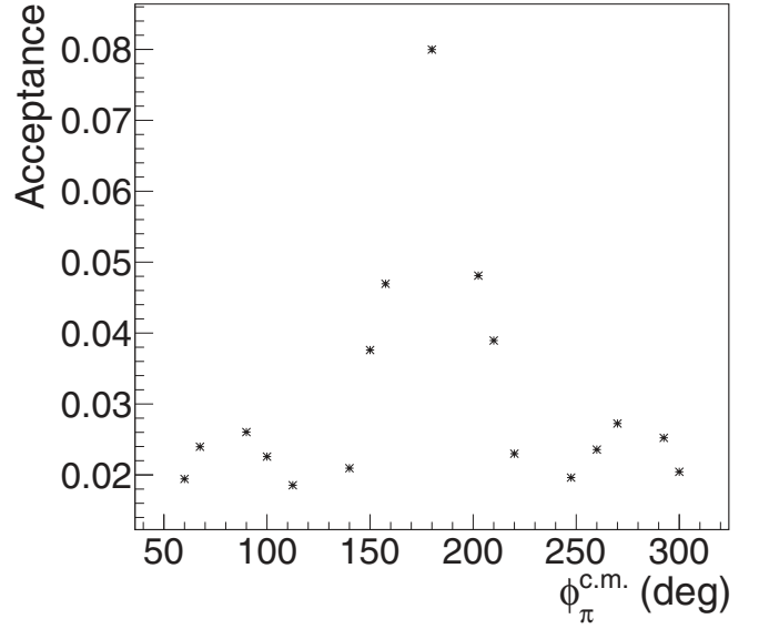
FIG. 20. Typical of acceptance correction factors as a function of \phi_{\pi^-}^{\text{c.m.}} for W = 1.2125 \text{ GeV} and Q^2 = 0.5 \text{ GeV}^2 , and \cos \theta_{\pi^-}^{\text{c.m.}} = 0.1 .
