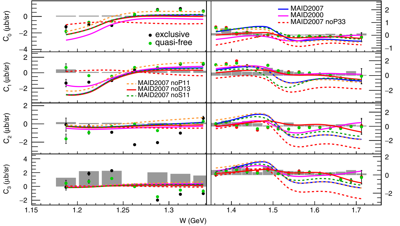
FIG. 33. The W -dependent Legendre moments C_i of \sigma_{LT} in Eq. (33) up to l_{\max} = 2 at Q^2 = 0.5 \text{ GeV}^2 that are extracted from the exclusive (black points) and quasifree (green squares) cross sections. For W > 1.35 \text{ GeV} , the rightmost y-axis scale is used. The data are compared with the MAID2007 [56] and MAID2000 [57] models. The solid lines represent the full model calculations. The dashed lines correspond to the MAID2007 model with specified resonant helicity amplitudes turned off [e.g., noP33 indicates turning off the \Delta(1232)3/2^+ contributions]. The gray bars represent the corresponding systematic uncertainties of the data.
