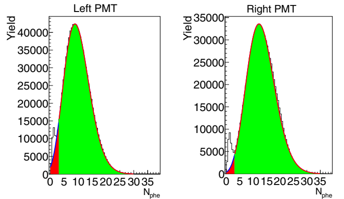
FIG. 8. N_{phe} histograms of the left and right PMTs in the tenth CC segment of sector 2 plotted separately and fit by the Poisson function in Eq. (11) shown by the red curve.
