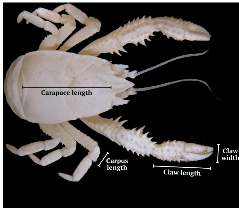
FIGURE 2 Morphological measurements of carapace length, claw length, claw width, and carpus length of the second pereopod in specimens of Kiwa puravida from Mound 12, Costa Rican Pacific margin. Scale bar: 0.5mm.
