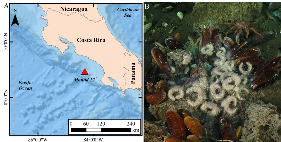
FIGURE 1 Sampling location (A) and detail of the yeti crabs Kiwa puravida (B) at Mound 12, a methane seep at ~1,000 m deep on the Costa Rican Pacific margin.
