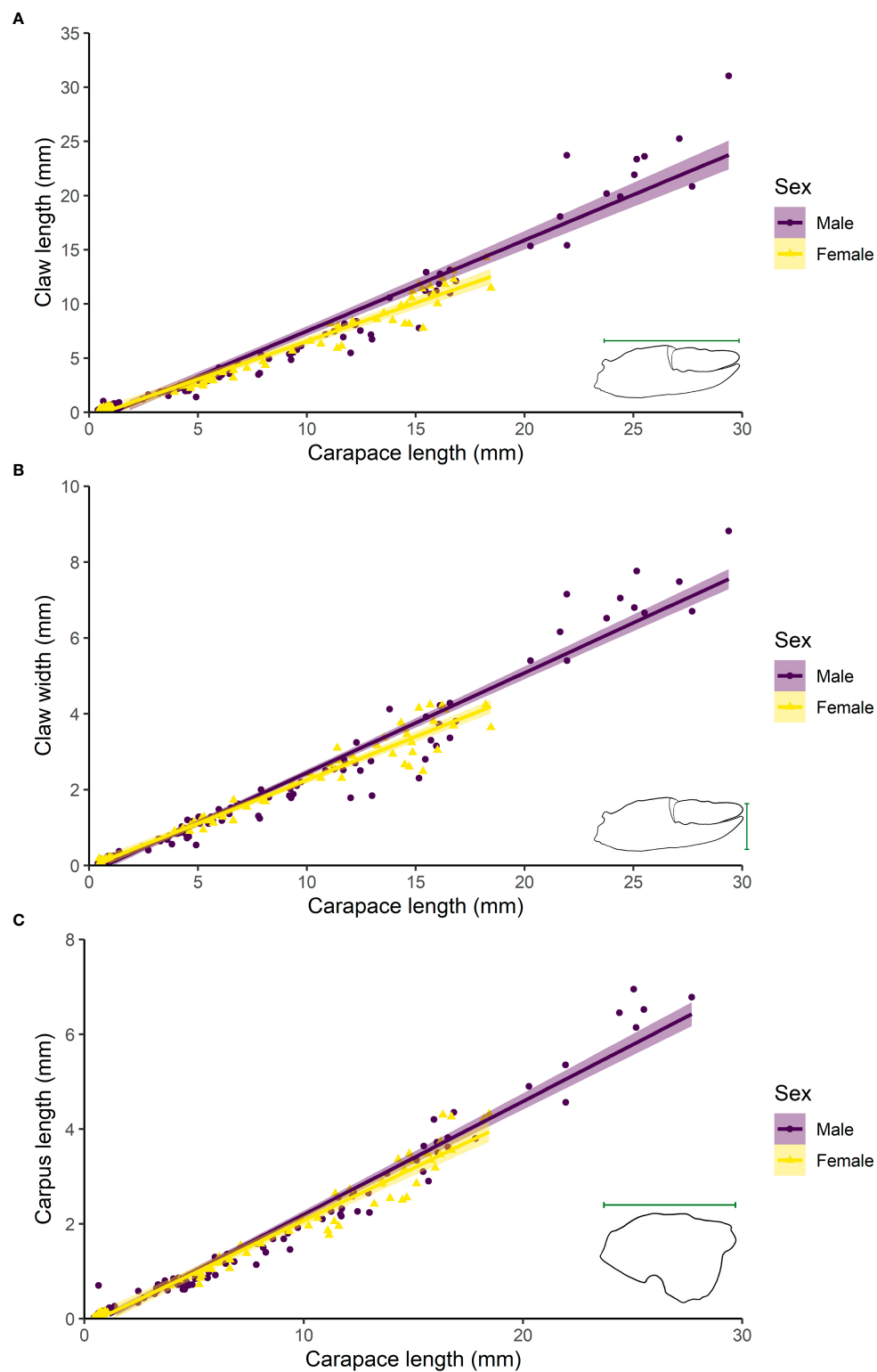
FIGURE 3 Comparison of the relationship of the claw length (A), claw width (B), and carpus length of the second pereopod (C) with the carapace length by sex (adult males and females) of Kiwa puravida , 2011 from Mound 12, Costa Rican Pacific margin. Data were fitted in linear regression models, shading represents 95% confidence interval around the model fit.
