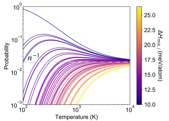
FIG. 3. Within a given ensemble, the variation in \Delta H_{\text{mix},i} leads to significant temperature evolution of the probability for each configuration. In the high-temperature limit, the probabilities converge to n^{-1} . Here, an ensemble of 50 \text{PbSe}_{0.5}\text{Te}_{0.5} configurations is considered, with each configuration represented by a line colored by its \Delta H_{\text{mix},i} .
