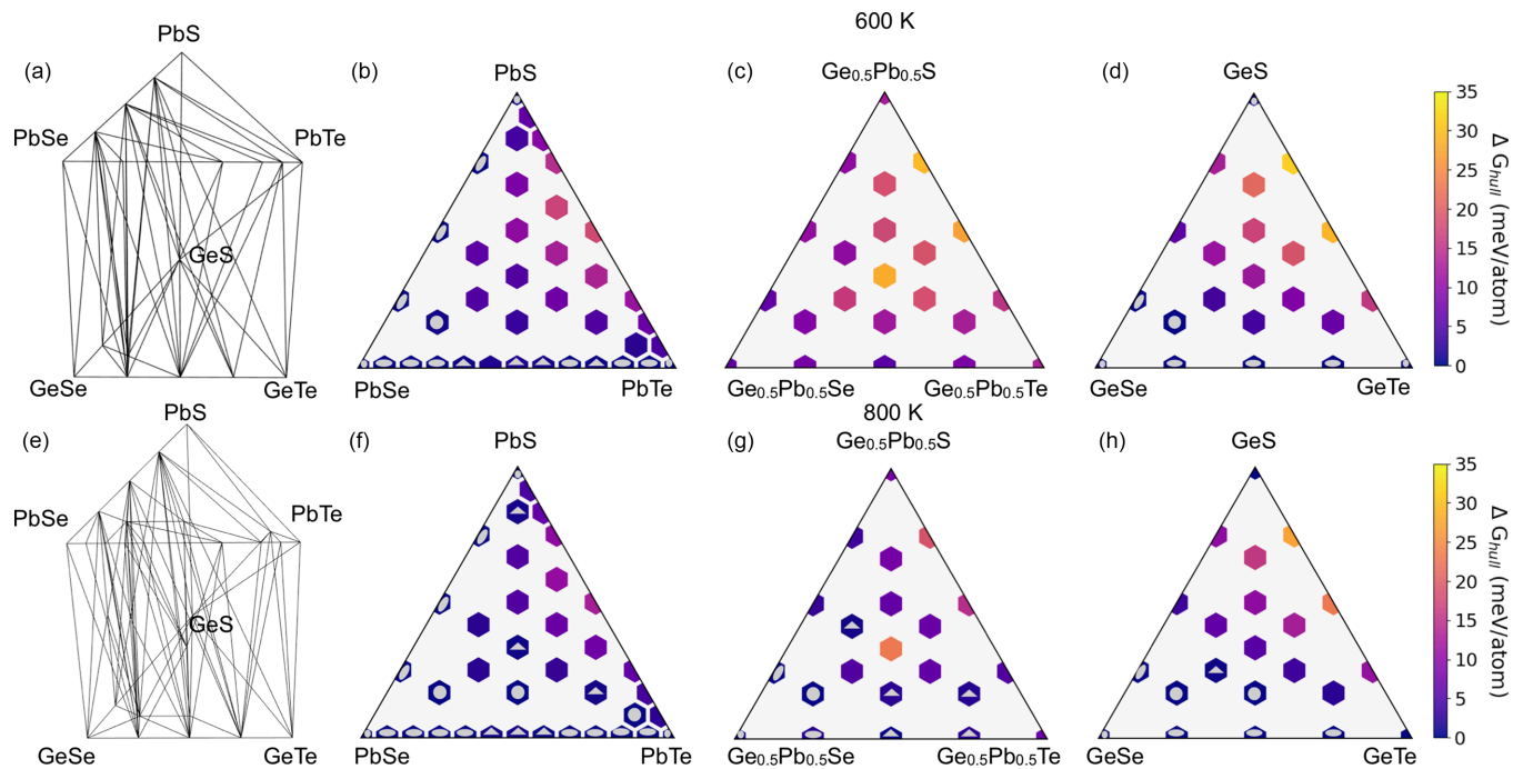
FIG. 12. (a) The (\text{Pb}_{1-x}\text{Ge}_x)(\text{Te}_y\text{Se}_z\text{S}_{1-y-z}) phase space is visualized as a prism with cation composition varying along the axis. Pseudoternaries (b)–(d) show three slices of this prism with discrete sampling; the color scheme denotes the free energy above the convex hull. Hexagons with a silver point inside indicate that they are on the hull; hexagons with a triangle denote compositions whose distance from the hull is less than their uncertainty ( 2\sigma_{E,n} , as determined by the CLT). Calculating the convex hull at 600 K using the coarse sampling of (b)–(d) fills the interior of the prism with four-phase tetrahedra. At this temperature, the x = 0.5 compositions are not on the hull, and the resulting tetrahedra of (a) span from x = 0 to 1 compositions. (e)–(h) The lower row shows the results at 700 K. At this temperature, far more compositions are on the hull, including in the interior of the prism (g), where many of the compositions exhibit significant entropy stabilization.
