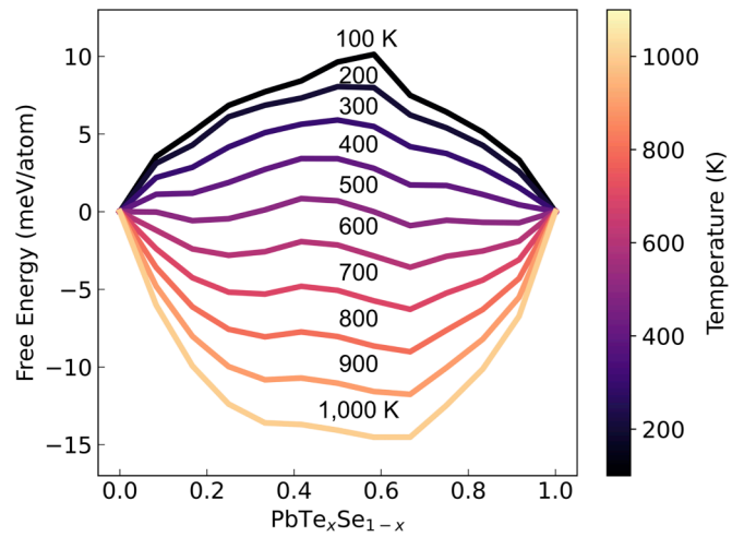
FIG. 9. The \Delta G_{\text{mix}} of \text{PbSe}_{1-x}\text{Te}_x gradually becomes more concave with increasing temperature, reaching full convexity at 700 K (within a tolerance of 2\sigma_{\Delta H,n} ). Here, the alloy compositions are sampled at 1/12 increments.
