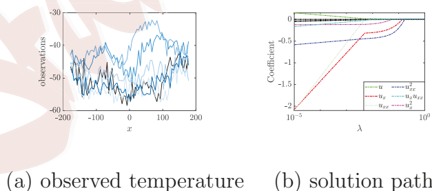
Figure 9: Visualization and identification of the CALIPSO data.
