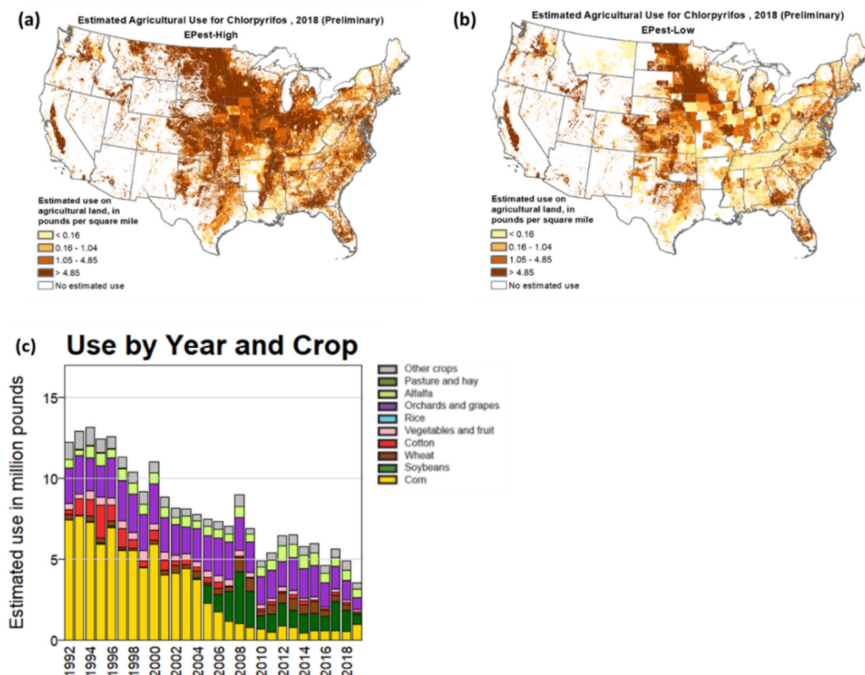
Figure 1. The map of estimated agricultural usage of chlorpyrifos in 2018: (a) Epest-high; (b) Epest-low; and (c) estimated usage for different crops from 1992 to 2018 [6].
