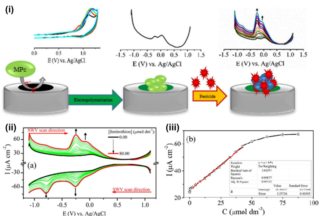
Figure 4. (i) Schematics of the electrochemical sensor fabricated by electropolymerization of metallophthalocyanines. (ii) SWV responses of GCE/CoPc(ma) during the titration with fenitrothion pesticide and (iii) its calibration line. These images were adapted from Akyüz et al. [130] with permission from Elsevier.
