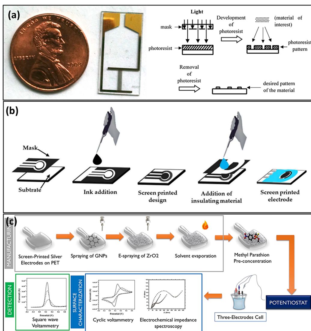
Figure 5. (a) Photolithographically-fabricated electrochemical sensor and schematic of the fabrication process. These images were adapted from Narakathu et al. [46], with permission from Elsevier and Park and Shuler [160] and with permission from John Wiley and Sons, respectively. (b) Manufacturing stages of SPEs [142], reproduced with permission from Pérez-Fernández et al., published by MDPI, 2020. (c) A fully roll-to-roll manufactured electrochemical sensor based on graphene nanoplatelet and ZrO 2 , reproduced with permission from reference [112], Copyright {2021} American Chemical Society.
