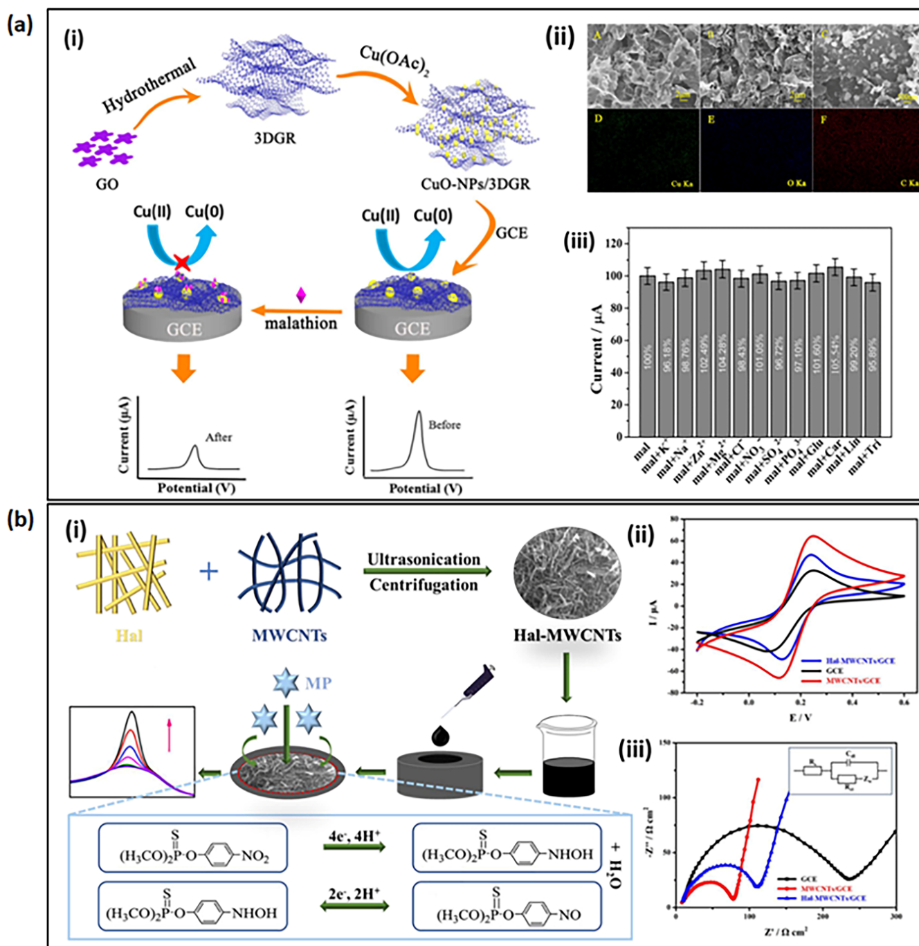
Figure 3. (a) (i) Schematics of the electrochemical detection of malathion using the fabricated CuO-NPs/3D graphene/glassy carbon electrode (GCE). (ii) Scanning electron microscopy (SEM) images of graphene, CuO-NPs/3DGR nanocomposite and CuO-NPs/3D graphene nanocomposite with their elemental mappings (iii) The bar graph that shows the selectivity of CuO-NPs/3D graphene/GCE without and with different interferences at a fixed concentration of malathion (1 nM). These images were adapted from Xie et al. [77], with permission from Elsevier. (b) (i) Schematics of the fabrication process of the Hal-MWCNTs/GCE electrochemical sensor and its mechanism to detect methyl parathion. (ii) Cyclic Voltammetry (CV) curves. (iii) Electrochemical Impedance Spectroscopy (EIS) plot of Hal-MWCNTs/GCE electrode compared to bare GCE and MWCNTs/GC electrodes. These images were adapted from Zhao et al. [86] with permission from Elsevier.
