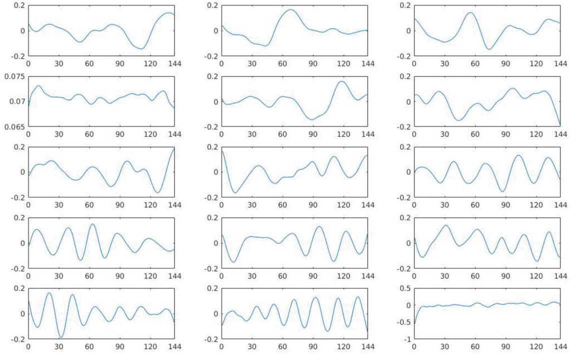
Figure 4. From left-to-right then top-to-bottom, we show the resulting first L = 15 eigenfunctions \hat{\phi}_k(t) estimated from the pooled empirical covariance function \hat{\Gamma}^*(s, t) .
