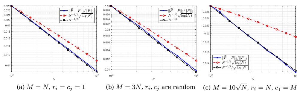
Figure 2: Empirical values of \|\tilde{P} - P\|_2 / \|P\|_2 as a function of N in log-log scale for the same settings as in Figure 1, compared to the corresponding bounds from (2.9).
