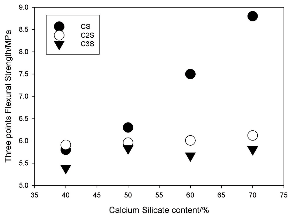
Fig. 8. Three-point flexural strength of inorganic polymer cement as a function of calcium silicate content.
