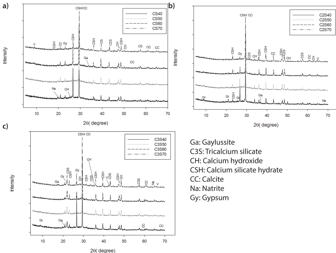
Fig. 1. XRD patterns of inorganic polymer cement: a) CS series, b) \text{C}_2\text{S} series, and c) \text{C}_3\text{S} series.
