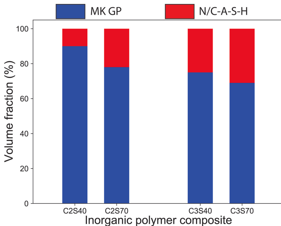
Fig. 14. Influence of calcium silicate content on the phase distribution of inorganic geopolymer composites. MK GP = amorphous metakaolin geopolymer. N/C-A-S-H = sodium/calcium aluminosilicate hydrates.
