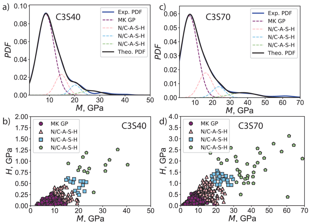
Fig. 13. Statistical deconvolution analysis of indentation data for inorganic polymer composites C 3 S 40 and C 3 S 70 . PDF = probability distribution function. M is the indentation modulus, and H is the indentation hardness. MK GP = amorphous metakaolin geopolymer. N/C-A-S-H = sodium/calcium aluminosilicate hydrates.
