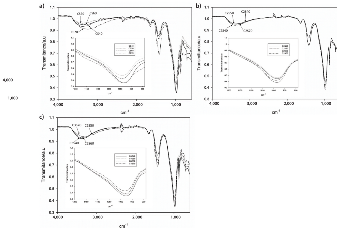
Fig. 2. FTIR spectra of inorganic polymer cement: a) CS series, b) C 2 S series, and c) C 3 S series.
