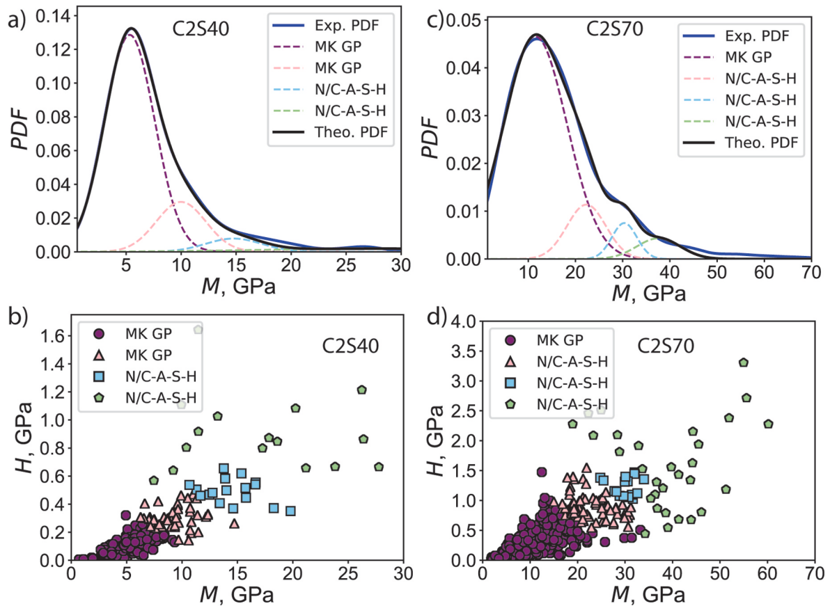
Fig. 12. Statistical deconvolution analysis of indentation data for inorganic polymer composites C 2 S 40 and C 2 S 70 . PDF = probability distribution function. M is the indentation modulus and H is the indentation hardness. MK GP = amorphous metakaolin geopolymers. N/C-A-S-H = sodium/calcium aluminosilicate hydrates.
