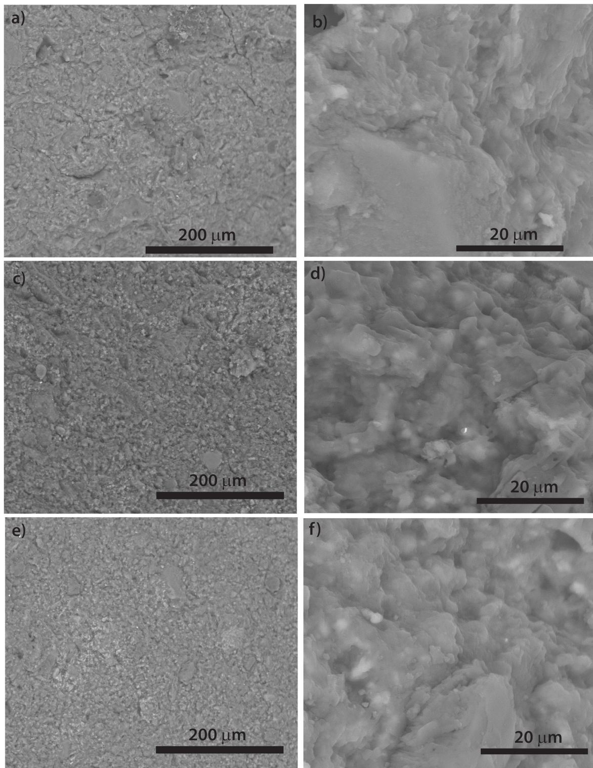
Fig. 6. Morphology of inorganic polymer cement: CS70 (a and b), C 2 S70 (c and d), C 3 S70 (e and f).
