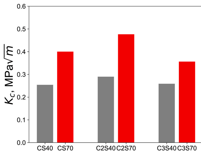
Fig. 10. Fracture toughness K_c of inorganic polymer composite specimens. N = 8 tests were conducted for each specimen.
