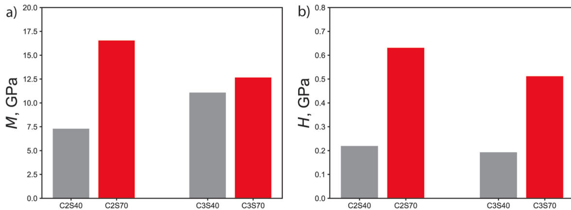
Fig. 9. Influence of calcium silicate content on elasto-plastic characteristics of inorganic geopolymers: a) average indentation modulus M . b) Average indentation hardness H for the tested specimens. N = 256 indentation tests were performed for specimens C2S40 and C3S40, and N = 441 indentation tests were performed for the remaining specimens.
