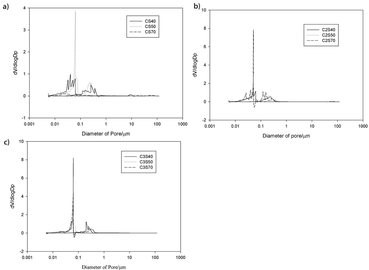
Fig. 5. Pore size distribution of inorganic polymer cement: a) CS series, b) C 2 S series, and c) C 3 S series.
