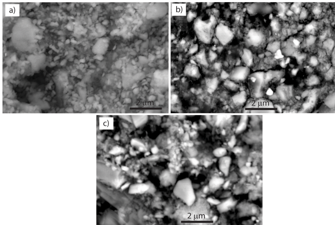
Fig. 7. Granular nature of inorganic polymer cement: a) CS70, b) C 2 S70, and c) C 3 S70.
