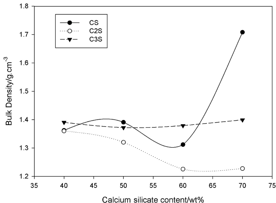
Fig. 3. Bulk density of inorganic polymer cement as a function of calcium silicate content.
