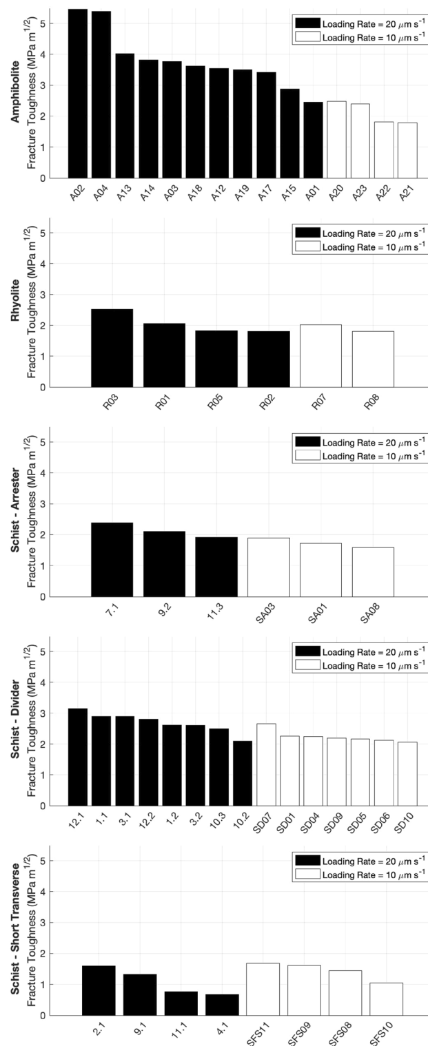
Figure 5. Fracture toughness values from all tests. Black bars indicate a loading rate of 20 \mu\text{m/s} , white bars indicate a loading rate of 10 \mu\text{m/s} .
