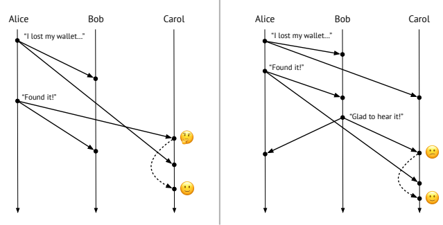
Figure 1: Two executions that violate causal delivery (Definition 2). On the left, Carol sees Alice’s messages in the opposite order of how they were sent. On the right, Carol sees Bob’s message before seeing Alice’s second message. The dashed arrows in both diagrams depict how a causal delivery mechanism (Section 2.2) might delay received messages in a buffer for later delivery.
