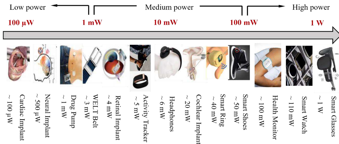
Figure 3. Typical average power consumption of wearable electronics [64–70].
