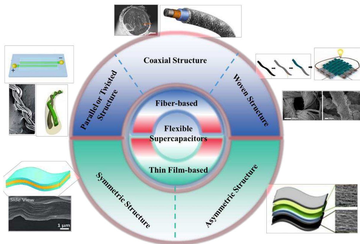
Figure 1. Types of flexible supercapacitors and their typical configurations. Images are adapted with permission from references [11,30–35].
