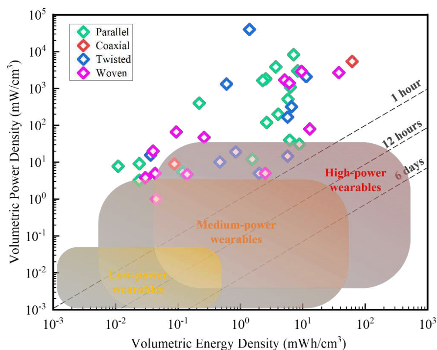
Figure 4. Ragone plot of reported energy and power densities of fiber-based flexible supercapacitors compared to the needs of typical wearable electronics.
