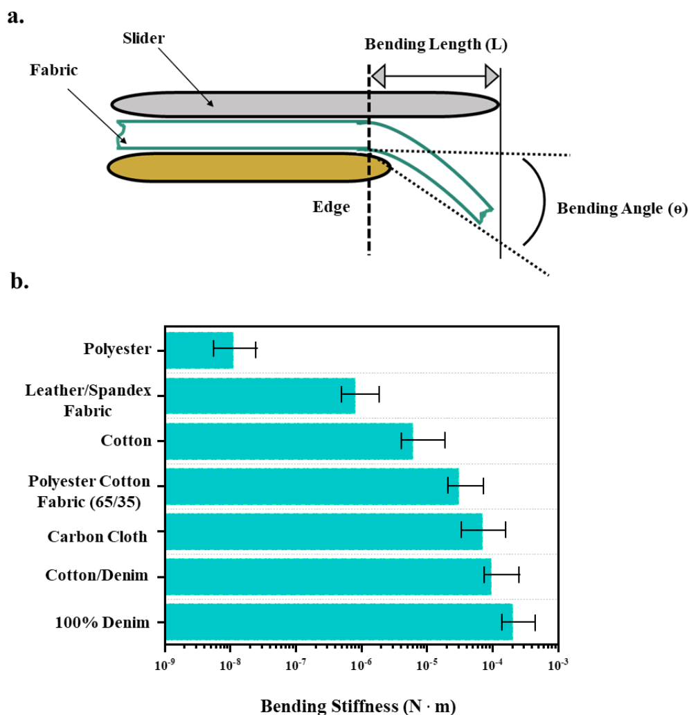
Figure 5. (a) Illustration of the bending stiffness test setup that is widely used in textile industry. (b) Typical bending stiffness values of commercial fabrics measured through the setup illustrated in (a) [110–114].
