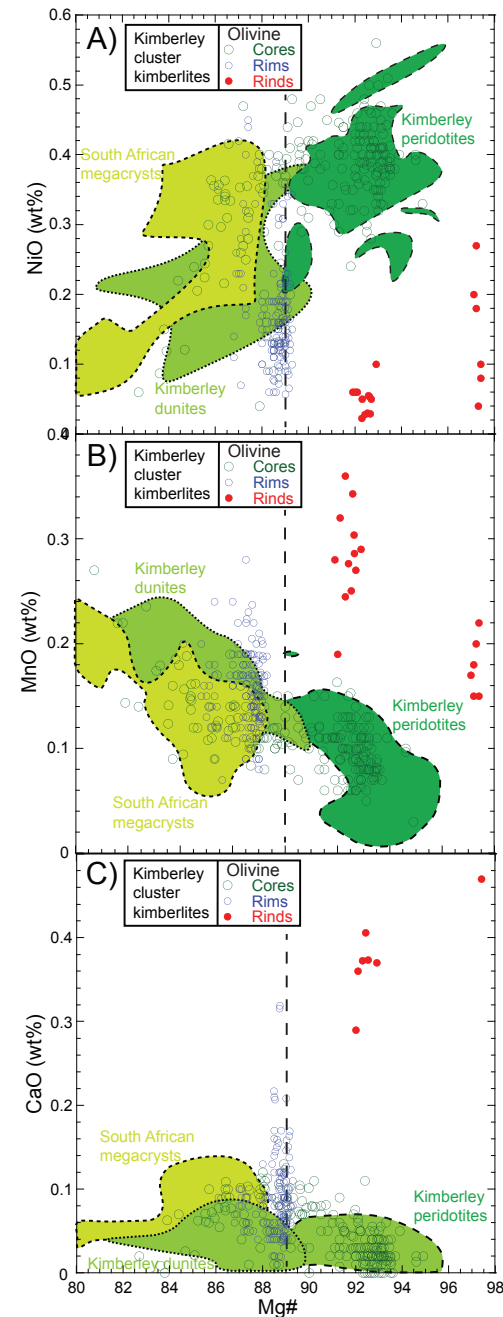
Figure 18. (A) Mg# vs NiO (B); Mg# vs MnO; (C) Mg# vs CaO for Kimberley cluster kimberlite-derived olivine macrocrysts cores, rims and rinds. Composition of olivine from coarse and sheared mantle peridotites, and olivine from dunites (interpreted as magmatic cumulates that are associated with the megacryst suite) from Kimberley cluster kimberlites are shown as fields. The field for southern African olivine megacrysts is also shown. All raw olivine data from Soltys et al. (2020).
