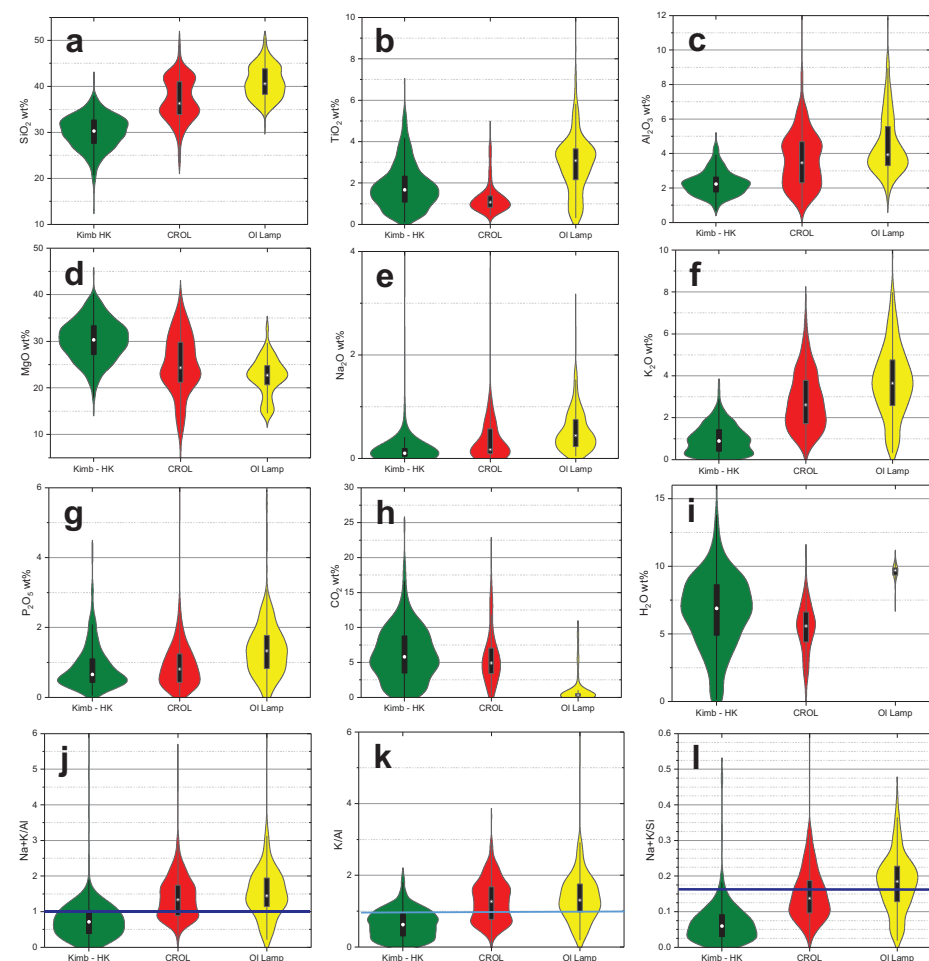
Figure 23. Kimb-HK, CROL, and olivine lamproite violin + box plots for (a) \text{SiO}_2 , (b) \text{TiO}_2 , (c) \text{Al}_2\text{O}_3 , (d) \text{MgO} , (e) \text{Na}_2\text{O} , (f) \text{K}_2\text{O} , (g) \text{P}_2\text{O}_5 , (h) \text{CO}_2 , (i) \text{H}_2\text{O} (j) (\text{Na}+\text{K})/\text{Al} , (k) \text{K}/\text{Al} , (l) (\text{Na}+\text{K})/\text{Si} . The blue lines in (j) divide alkaline ( >1 ) and subalkaline ( <1 ) samples. The blue line in (k) demarcates samples with \text{K}/\text{Al} > 1 (perpotassic). The blue line in (l) demarcates samples with (\text{Na}+\text{K})/\text{Si} > 0.1666 that are considered alkaline on the basis of a silica deficiency with respect to alkalis. See text for further discussion. The box and line plot showing the median ( white circle ) and the interquartile range (50% of the data—the box, in black ) with the lines representing the upper and lower quartiles of the data; this is combined with a “violin” plot, which is in essence a probability density function of the data. The sources of the data are in the on-line appendix A.
