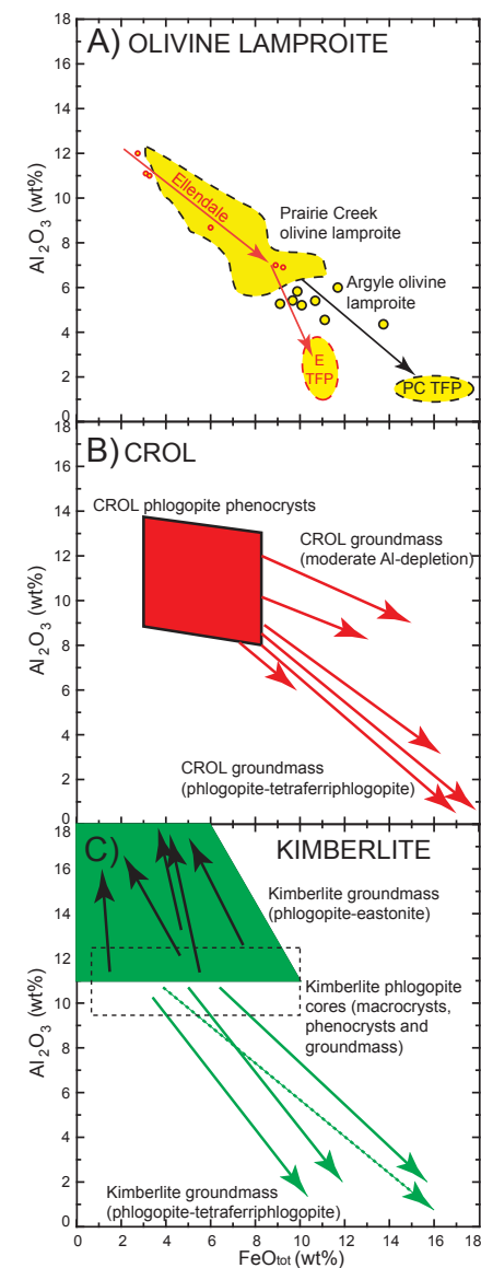
Figure 17. Bivariate plot of \text{Al}_2\text{O}_3 versus \text{FeO}_{\text{total}} for phlogopite mica from (A) olivine lamproites, (B) CROL, and (C) kimberlites. For olivine lamproites and CROLs, zoning trends are from phenocryst cores to rims and groundmass grains; both these rock types exhibit phlogopite with moderate-Al depletion- and extreme-Al depletion (to TFP) trends. Kimberlite zoning trends can be observed within only groundmass grains, and as phlogopite cores (macrocrysts, phenocrysts, micro-phenocrysts) with compositional zoning to the margins. See text for details and data sources.
