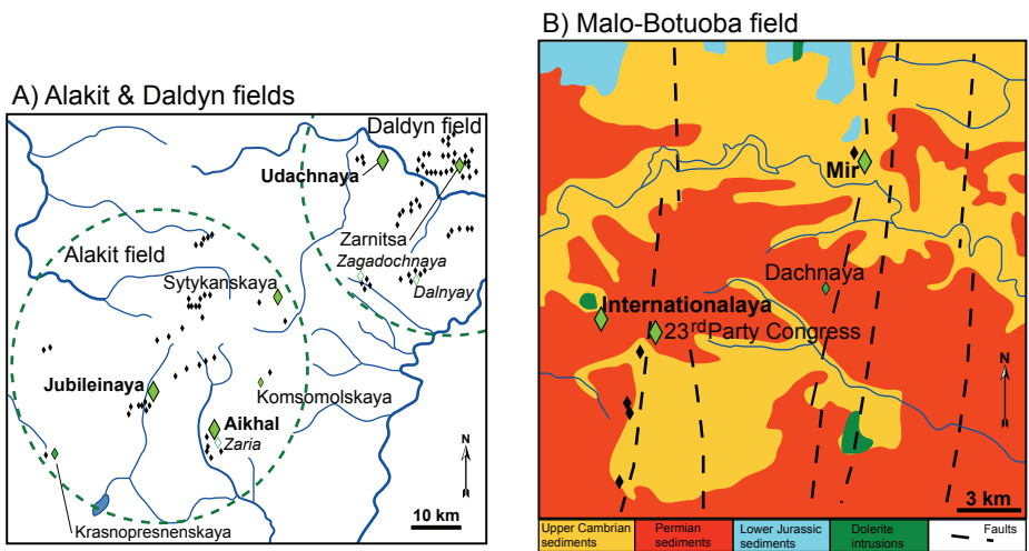
Figure 28. Detail maps of Siberian Craton kimberlites and kimberlite-hosted diamond mines, deposits and advanced exploration projects. Tier 1 diamond mines indicated by bold font. Mine data from Table 2. (A) Alakit-Markha and Daldyn kimberlite fields (modified after Ashchepkov et al. 2015 and Kostrovitsky et al. 2015). (B) Malo-Botuoba field (modified after Agashev et al. 2018).
