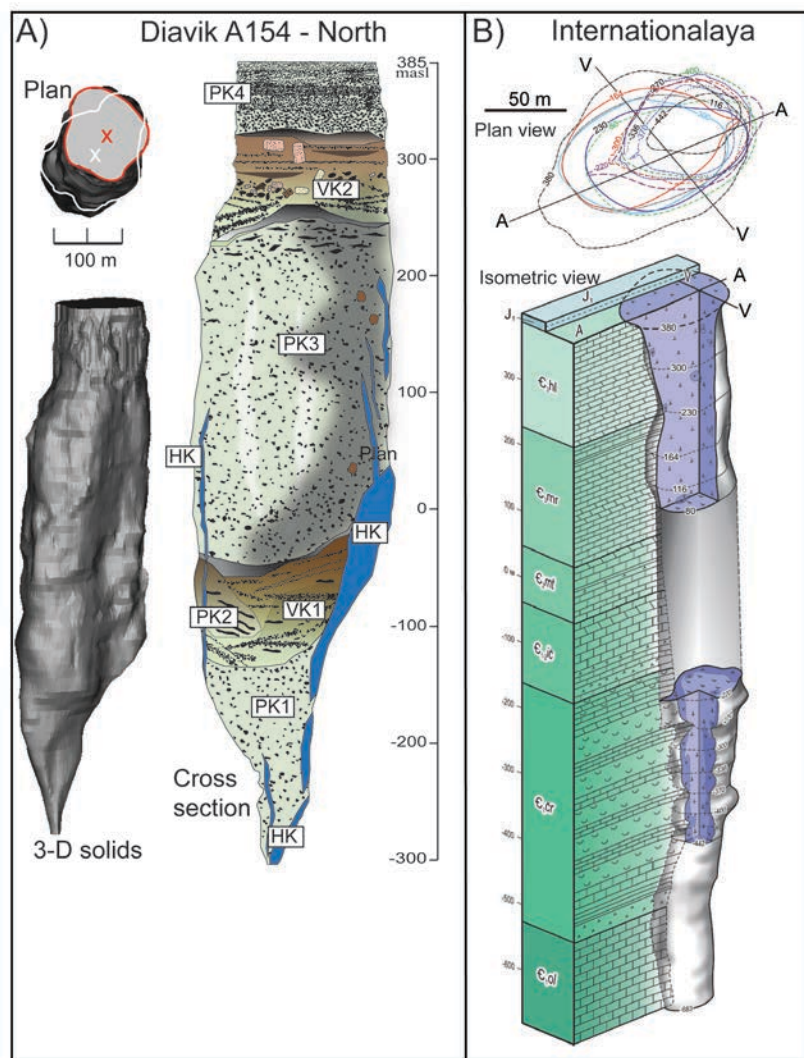
Figure 11. (A) Plan and 3-D solids and cross section of the A154—North kimberlite, Diavik Mine, Lac de Gras kimberlite field, NT, Canada. Note the multiple phases of kimberlite in the A154 North cross section. HK = hypabyssal kimberlite; PK1, PK2, PK3 = pyroclastic kimberlite phases 1, 2, 3; VK1, VK2 = volcaniclastic kimberlite phases 1 and 2. After Moss et al. (2018), with permission. (B) The steep-walled Internationalaya, Russia kimberlite, plan and isometric views. After Kostrovitsky et al. (2015), with permission.
