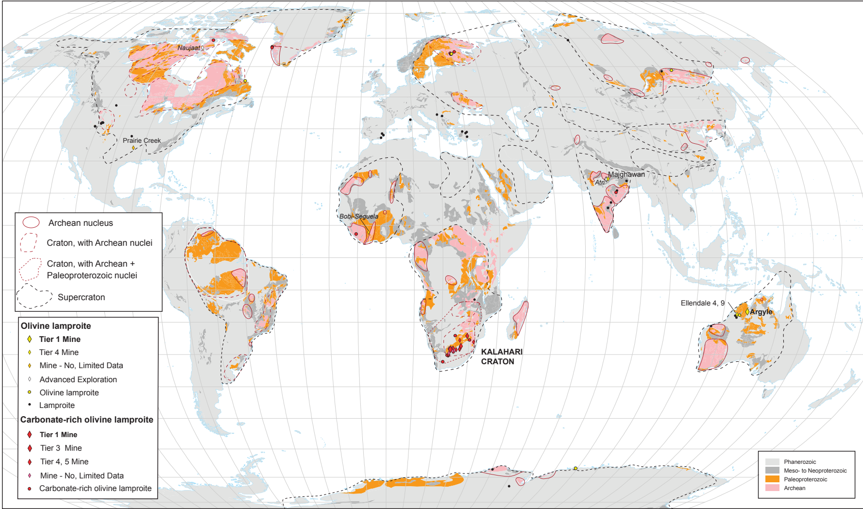
Figure 2. Global distribution of CROL- and olivine lamproite-hosted diamond mines, past producing mines and advanced exploration projects. Additional CROLs, olivine lamproites and lamproites (e.g., leucite lamproites, Mediterranean lamproites) locations show the main fields and clusters globally. Bedrock geology backdrop from Chorlton (2007); note the dominant bedrock geology is that at the surface i.e., Phanerozoic rocks that overlie Archean or Proterozoic rocks are shown on this map as Phanerozoic. Craton outlines from Pearson et al. (2021). Robinson map projection.
