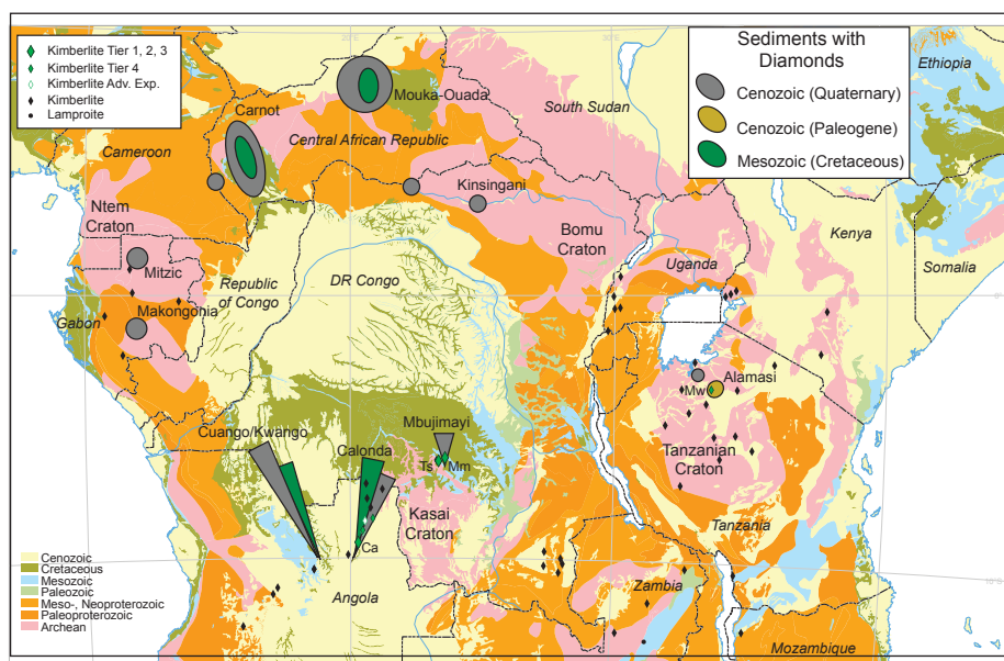
Figure 64. Central Africa placer deposits as labeled on the map (Mouka-Ouadda, Carnot, Mitzi, Makongonia, Cuango/Kwango River, Calonda, Mbuji Mayi, Alamasi, Kinsangani). Primary magmatic kimberlite mines/deposits as follows: Ca, Catoca; Ts, Tschibwe; Mm, Mbuji Mayi, Mw, Mwadui. Mercator map projection.
