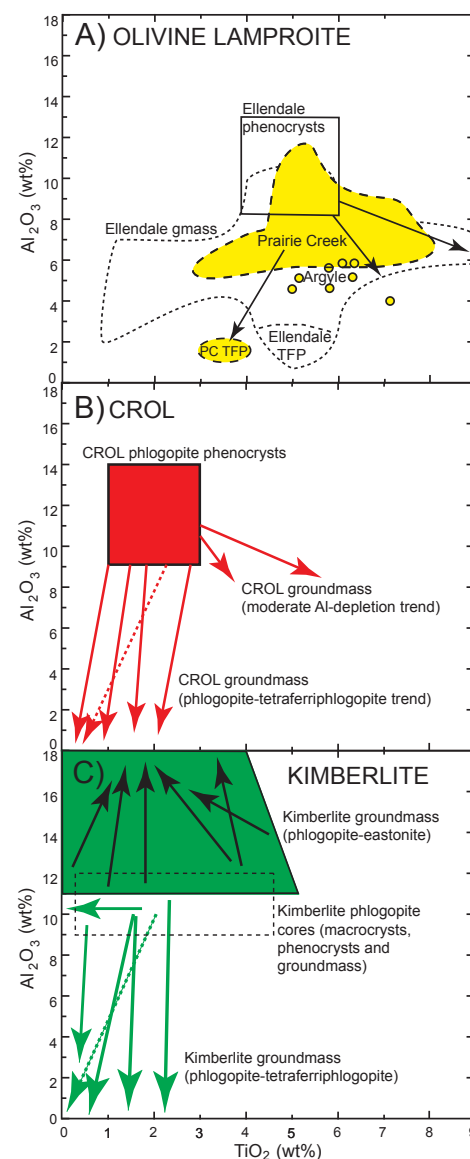
Figure 16. Bivariate plot of \text{Al}_2\text{O}_3 versus \text{TiO}_2 for phlogopite mica from (A) olivine lamproites, (B) CROL, and (C) kimberlites. For olivine lamproites and CROLs, zoning trends are from phenocryst cores to rims and groundmass grains; both these rock types contain phlogopite that exhibit moderate- and/or extreme-Al depletion trends. Kimberlite zoning trends can be observed within groundmass grains, and as phlogopite cores (macrocrysts, phenocrysts, micro-phenocrysts) with compositional zoning to the margins. In kimberlites, phlogopite Al-enrichment and Al-depletion trends are observed. See text for details and data sources.
