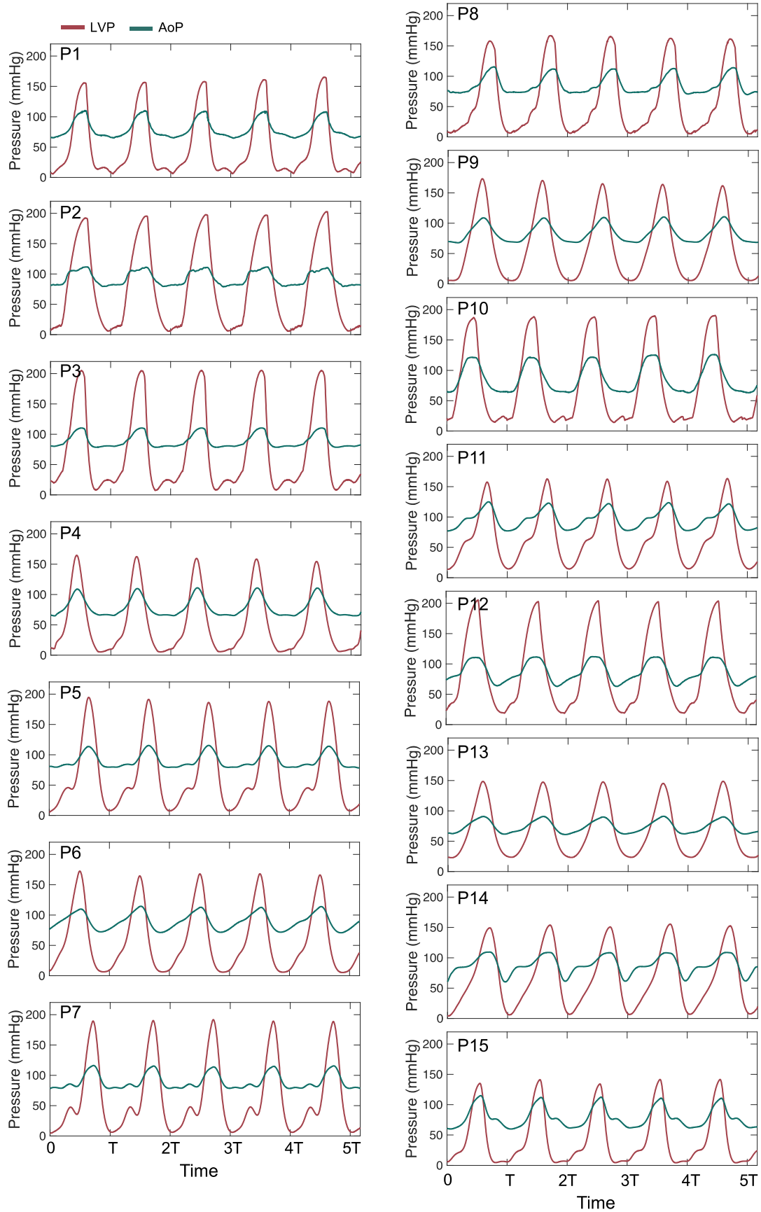
Fig. S5. Pressure waveforms obtained through the soft robotic model. Overlaid left ventricular pressure (LVP) and aortic pressure (AoP) waveforms from catheterization data on soft robotic model for n = 5 consecutive heartbeats for patients 1-15.
