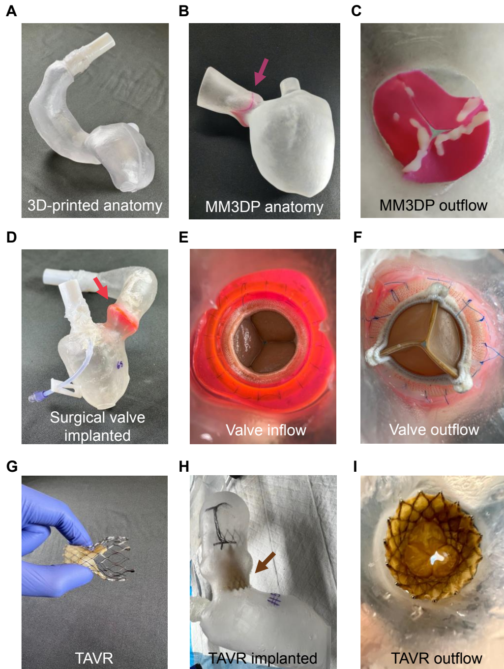
Fig. S4. Illustration of 3D printing methods and use of surgical and TAVR valves. (A) 3D-printed anatomy of the LV and aorta of use for soft robotics-driven model. (B) Multi-material 3D-printed (MM3DP) anatomy of the LV, aorta, and aortic valve (arrow). (C) Details of the MM3DP valve outflow. (D) Surgical valve implanted (arrow) in 3D-printed anatomy to recreate physiologic aortic hemodynamics, with details of the implanted valve (E) inflow and (F) outflow. (G) View of the Evolut R (Medtronic) self-expandable TAVR. (H) TAVR implanted (arrow) in the 3D-printed anatomy. (I) Detail of the TAVR in outflow view.
