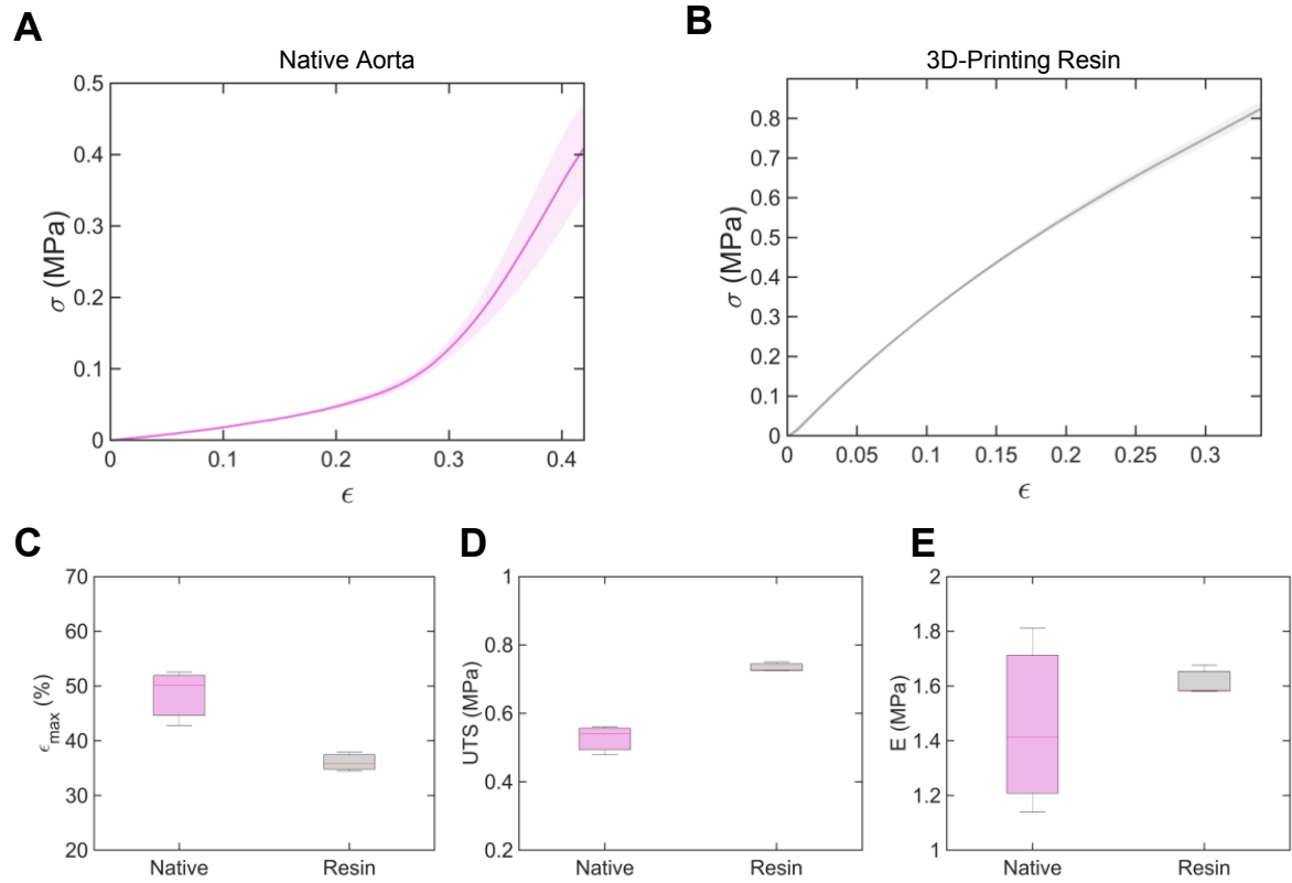
Fig. S1. Mechanical characterization of the native porcine aorta and 3D-Printing resin. Stress-strain raw data of (A) the native aorta and of the (B) the 3D-printing resin. Mechanical testing was performed using an electromechanical tester (Instron 5566, 50N load cell, Norwood, USA), and dogbone-shaped specimens subjected to uniaxial loading at a rate of 2 mm/min according to the American Society for Testing and Materials (ASTM) standards. Graphs show mean \pm 1 s.d. ( n = 3 ). (C) Maximum specimen elongation at failure, (D) Ultimate tensile strength (UTS), (E) Young's modulus for three different specimens of the native aorta and the resin ( n = 3 ). Young's modulus was calculated in the 25-35% strain interval. \sigma : engineering stress, \epsilon : engineering strain, E: Young's modulus.
