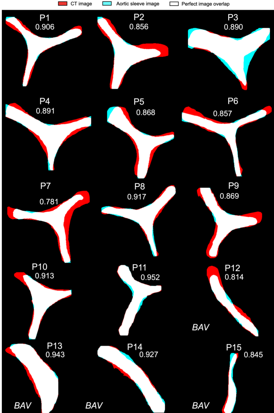
Fig. S3. Comparison of aortic stenosis morphologies obtained by computed tomography (CT) and actuation of the soft robotic aortic sleeve. Images for all the 15 patients (Patients 1-15) were binarized and cross-registered. White regions correspond to a perfect overlap between each pair of images, while cyan or red regions correspond to areas of noncongruent geometries. For each pair of images, the DSC was computed and was reported below the corresponding patient number. BAV: bicuspid aortic valve.
