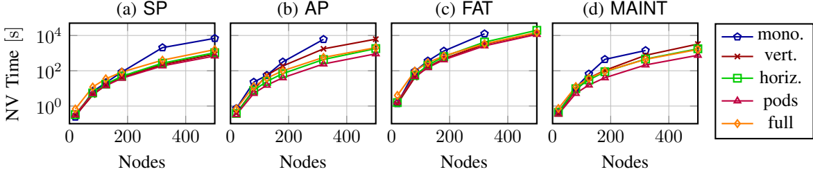
Fig. 8: NV times for fattree benchmarks.
