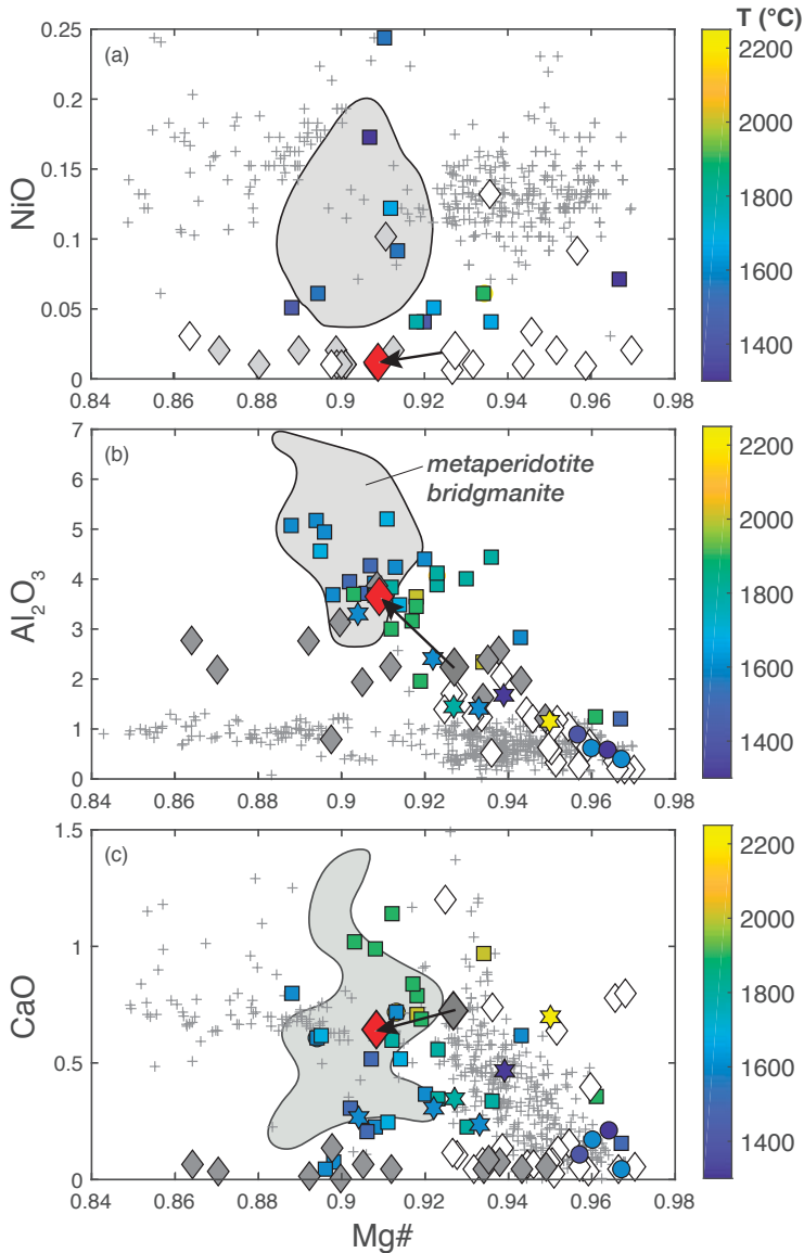
Figure 14. NiO (a), \text{Al}_2\text{O}_3 (b) and CaO (c) versus Mg# showing \text{MgSiO}_3 -rich inclusions: white diamonds , low-Al single phase inclusions; light grey diamonds in (a) are high-Al inclusions. In (b) and (c) dark grey diamonds are low-Al composite inclusions; red diamond , re-constructed low-Al, high Ca inclusion from Burnham et al. (2016), connected to the measured \text{MgSiO}_3 portion of the inclusion by an arrow. Experimental bridgmanites coexisting with ferropericlase \pm Ca-silicate perovskite in meta-peridotitic assemblages are shown as a light grey field (Ito and Takahashi 1987; Irifune 1994; Wood 2000; Hirose 2002; Tronnes and Frost 2002; Nishiyama and Yagi 2003; Nishiyama et al. 2004; Walter et al. 2004; Irifune et al. 2010; Ishii et al. 2011, 2018, 2019; Kuwahara et al. 2018); squares , bridgmanite in experiments on meta-peridotite coexisting with majorite \pm ferropericlase / Ca-silicate perovskite / ringwoodite; circles , akimotoite in experiments on meta-peridotitic compositions coexisting with majorite \pm Ca-silicate perovskite / ringwoodite / stishovite; six pointed stars , bridgmanite in experiments on harzburgite composition; crosses , orthopyroxene inclusions in lithospheric diamonds (see Stachel et al. 2022 for references). Experiments denoted by symbols are shaded for experimental temperature.
