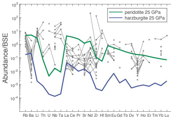
Figure 19. Trace element abundances in ferropericlasite inclusions from the global dataset normalized to BSE. Also shown are calculated abundance patterns for ferropericlasite expected in meta-peridotite (bridgmanite + Ca-silicate perovskite + ferropericlasite) and meta-harzburgite (bridgmanite perovskite + ferropericlasite) in the lower mantle at 25 GPa. Mineral modes and partition coefficients are provided in Table 3.
