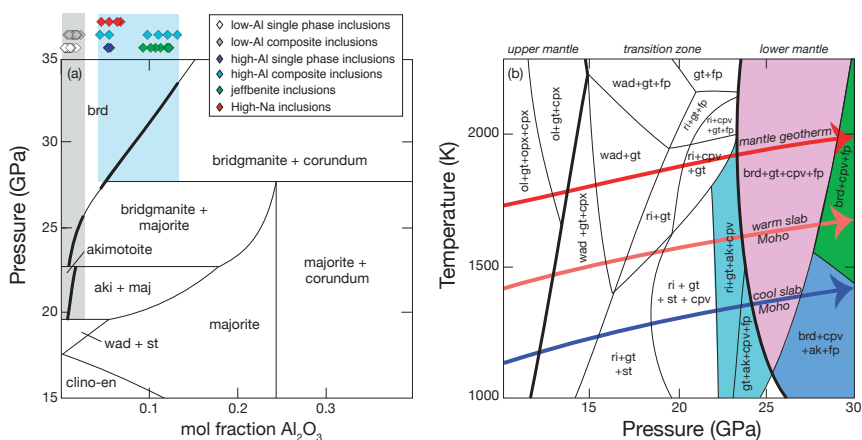
Figure 16. (a) Phase relations in the system \text{MgSiO}_3\text{-Al}_2\text{O}_3 (mole fraction \text{Al}/(\text{Al}+\text{Mg}) ) as a function of pressure at 1600 °C (Stixrude and Lithgow-Bertelloni 2011). Also shown are the alumina contents of the \text{MgSiO}_3 -rich inclusions (see symbol key). The grey bar shows the range of Al-content in low-Al inclusions and the blue bar the range in high-Al inclusions. (b) Phase relations for ‘pyrolitic’ mantle (Stixrude and Lithgow-Bertelloni 2011). The cyan region shows akimotoite + majoritic garnet stability, the purple shaded region shows bridgmanite + majoritic garnet stability, the dark blue region shows bridgmanite + akimotoite stability, and the green region bridgmanite stability. Also shown are model geotherms for the mantle (Katsura et al. 2010) and warm and cool slabs at the Moho (Shirey et al. 2021) (deflections at phase boundaries omitted). Phase labels are: ak = akimotoite; brd = bridgmanite; cpx = clinopyroxene; cpv = Ca-silicate perovskite; fp = ferropericlase; gt = garnet; ol = olivine; opx = orthopyroxene; ri = ringwoodite; st = stishovite; wad = wadsleyite.
