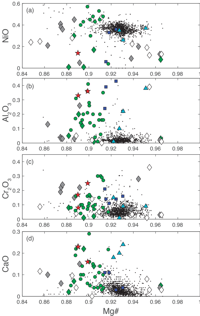
Figure 20. (a) NiO, (b) \text{Al}_2\text{O}_3 , (c) \text{Cr}_2\text{O}_3 and (d) CaO versus Mg# showing olivine inclusions from the global dataset: green diamonds , co-occurring with ferropericlase, \text{MgSiO}_3 , \pm\text{CaSiO}_3 ; grey diamonds , co-occurring with ferropericlase \pm\text{cpx} \pm\text{jeffbenite} ; white diamonds , other; crosses , olivine inclusions in lithospheric diamonds (see Stachel et al. 2022, this volume for references); green circles , experimental ringwoodite in meta-peridotite; red stars , experimental ringwoodite coexisting with akimotoite; blue squares , experimental wadsleyite in meta-peridotite; cyan triangles , experimental olivine in meta-peridotite at 13–14 GPa in equilibrium with majoritic garnet \pm\text{cpx} (Irifune and Ringwood 1987; Irifune 1994; Wood 2000; Hirose 2002; Ishii et al. 2011, 2018, 2019).
