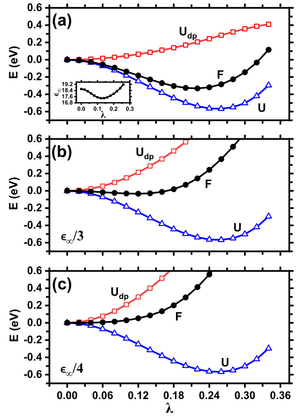
FIG. 3. (a) Electric free energy F(\lambda) (solid dots), internal energy U(\lambda) (empty triangles), and depolarization energy U_{dp}(\lambda) (empty squares) in -2\% strained LiZnSb under OCBC as a function of \lambda . The calculated high-frequency dielectric constant \epsilon_\infty(\lambda) is shown in the inset. (b) The same as (a), except that \epsilon_\infty is artificially reduced to 1/3 of its original value. (c) The same as (a), except that \epsilon_\infty is reduced to 1/4 of its original value.
