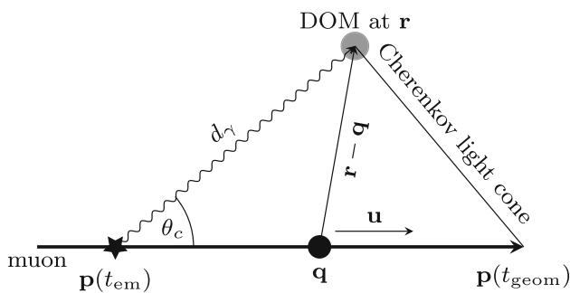
Fig. 5 Detailed geometry of a light cone created by a track. \mathbf{q} is the position of the anchor point and \mathbf{r} is the position of the optical module. \mathbf{p}(t_{\text{em}}) and \mathbf{p}(t_{\text{geom}}) are the positions of the muon at the time the photon is emitted and when it is geometrically expected to arrive, respectively
