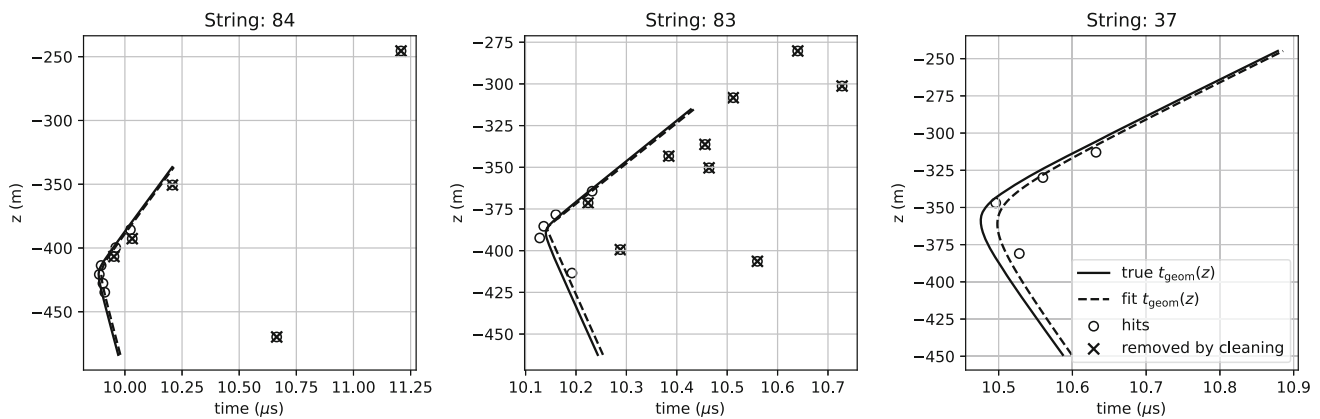
Fig. 4 Example of a \nu_{\mu}^{\text{CC}} event reconstructed with SANTA with hits on several strings. Strings 84, 83 and 37 are spaced \sim 80 m apart from each other and form a highly obtuse triangle
