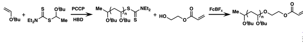
Figure 4. Through a) chain extension with methyl acrylate and b) post-polymerization functionalization to install an acrylate, cationic and radical RAFT can be combined to access a variety of polymer compositions and architectures.
