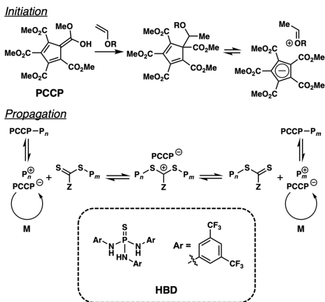
Figure 1. Proposed initiation and propagation for degenerate chain transfer with PCCP.
