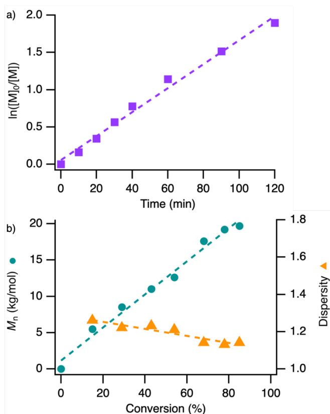
Figure 2. a) Semilogarithmic plot showed first order kinetics, indicating a constant concentration of propagating cations throughout the polymerization. b) Molecular weight increased linearly, and dispersity decreased with increased conversion. Hence, kinetic analysis suggested that the polymerization has living characteristics.
