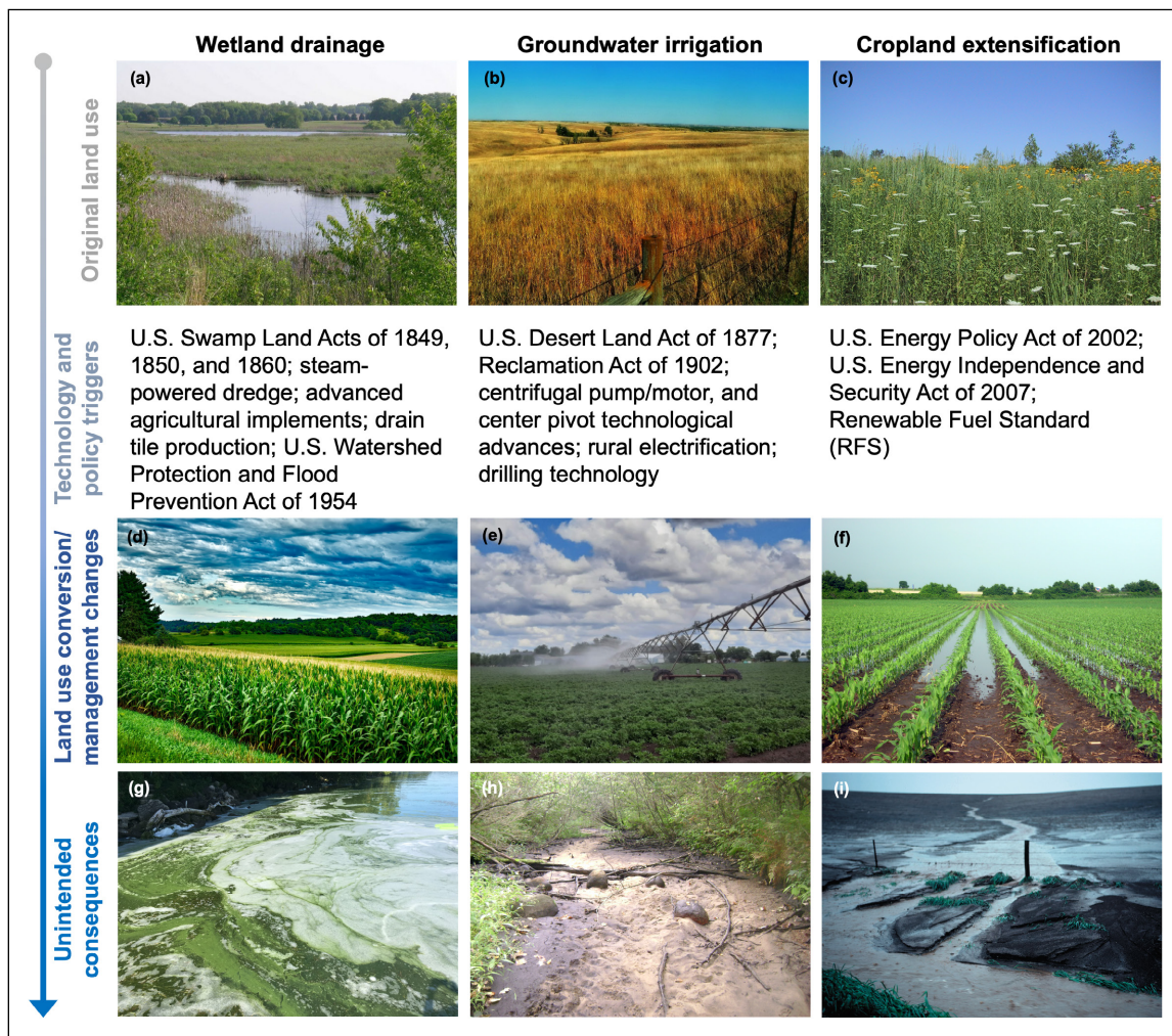
Figure 2. Land-use change and unintended consequences in the MRB. Technological and policy-based triggers (text beneath images in top row) that promoted wetland drainage, groundwater extraction for irrigation, and use of food crops for biofuel within a symbolic (a) wetland, (b) grassland, and (c) land enrolled in the Conservation Reserve Program (CRP), respectively. These triggers led to (d) increased row crop area after wetland drainage, (e) widespread use of groundwater irrigation, and (f) conversion of CRP to corn on marginal land. Unintended consequences include (g) algal blooms; (h) dry rivers and streams, and lower groundwater tables; and (i) increased soil erosion and runoff. Image credits: (f) S Zipper, (g) E Stanley, and (h) Center for Watershed Science and Education (University of Wisconsin–Extension).
