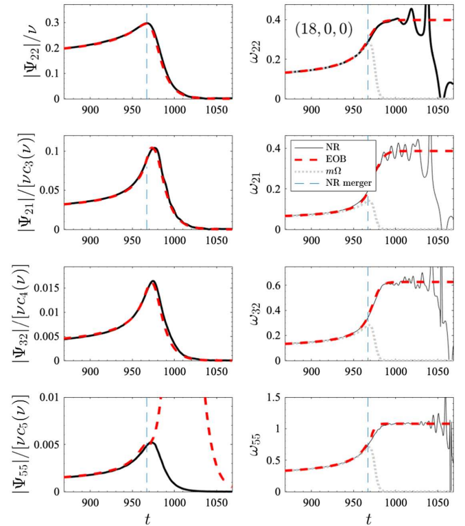
FIG. 6. EOB/NR comparison for q = 18 using the NR data of Ref. [87]. The unphysical behavior of the \ell = m = 5 mode after merger is evident.
