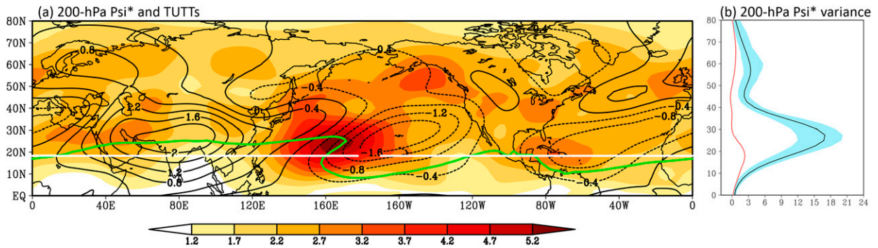
FIG. 1. (a) Long-term (1979–2018) mean 200-hPa \Psi^* (contours; 10^7 \text{ m}^2 \text{ s}^{-1} ), interannual standard deviation of 200-hPa \Psi^* (shaded; 10^6 \text{ m}^2 \text{ s}^{-1} ), 1 \text{ m s}^{-1} climatological zonal geostrophic wind ( U_g ) contour (green line), and the reference latitude (white line) during July–October. Here the reference latitude is defined as the averaged latitude of climatological 1 \text{ m s}^{-1} U_g contour, and the area where the circumglobal 1 \text{ m s}^{-1} U_g contour extends southward of the reference latitude represents climatological Pacific and Atlantic TUTTs (see text in section 2a for details). (b) The long-term mean wave amplitude ( 10^{13} \text{ m}^4 \text{ s}^{-2} ), 5th–95th percentile range of the seasonal-mean value ( 10^{13} \text{ m}^4 \text{ s}^{-2} ), and the 40-yr trend [ 10^{13} \text{ m}^4 \text{ s}^{-2} (40 \text{ yr})^{-1} ] are denoted by the black line, blue shading, and red line, respectively.
