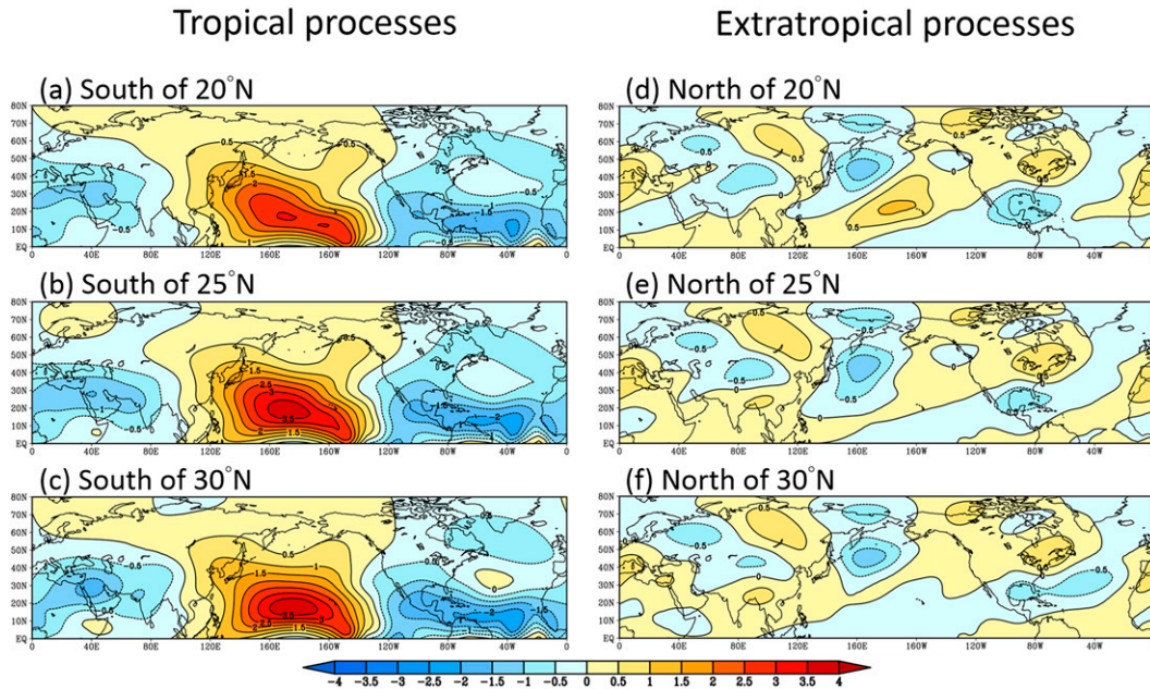
FIG. 11. Responses of 200-hPa \Psi^* to changes in diabatic heating and transient forcing south of (a) 20°N, (b) 25°N, and (c) 30°N, individually. (d)–(f) As in (a)–(c), but north of 20°, 25°, and 30°N, respectively. In the experiments focusing on the tropical processes [i.e., (a)–(c)], variations in transient forcing and diabatic heating are set to zeros north of different dividing latitudes, whereas these are prescribed as zeros south of the dividing latitudes in the extratropical processes simulations [i.e., (d)–(f)].
