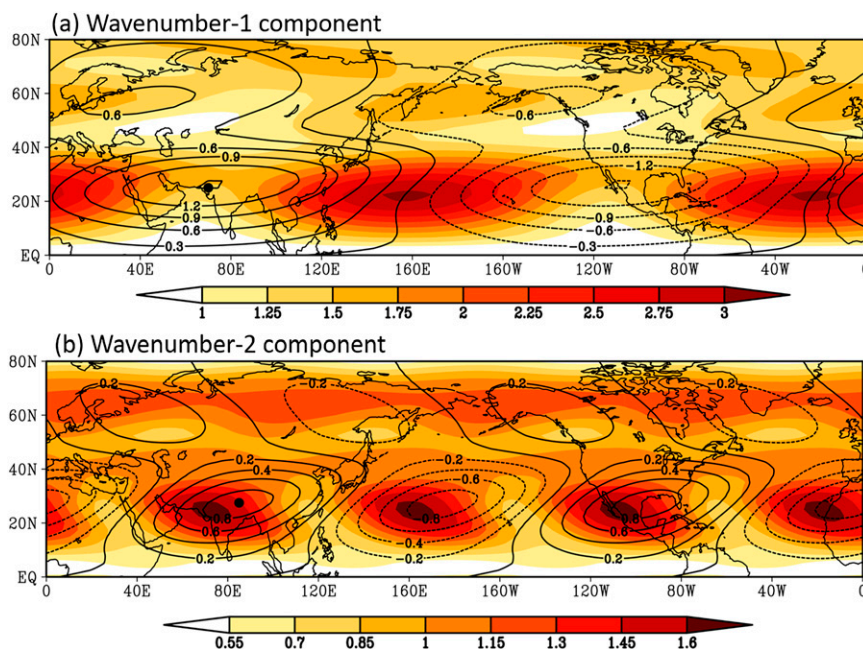
FIG. 3. Long-term mean (contours; 10^7 \text{ m}^2 \text{ s}^{-1} ) and interannual variability (shaded; 10^6 \text{ m}^2 \text{ s}^{-1} ) of 200-hPa \text{Psi}^* for (a) WN1 and (b) WN2, respectively. Central positions of WN1 and WN2 are denoted by the black dots, respectively.
