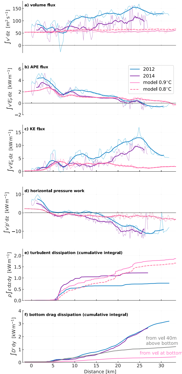
FIG. 10. Layer-integrated terms of the energy equation in observations and model. Model data are shown for one snapshot in time. Layer interfaces are defined by the 0.9^{\circ} and 0.8^{\circ}\text{C} isotherm for the model and the \sigma_4 = 45.94 \text{ kg m}^{-3} isopycnal for the towyo observations. (a) Volume flux per unit width calculated as vertical integral of horizontal velocities within the dense bottom layer. Thick lines here and in the following three panels show a 2-km windowed moving average, thin lines show results at each towyo profile or model grid point, respectively. (b) Horizontal flux of available potential energy. (c) Horizontal flux of kinetic energy. (d) Horizontal pressure work. (e) Turbulent dissipation cumulatively integrated horizontally and within the dense bottom layer. (f) Cumulative integral of dissipation caused by bottom drag.
