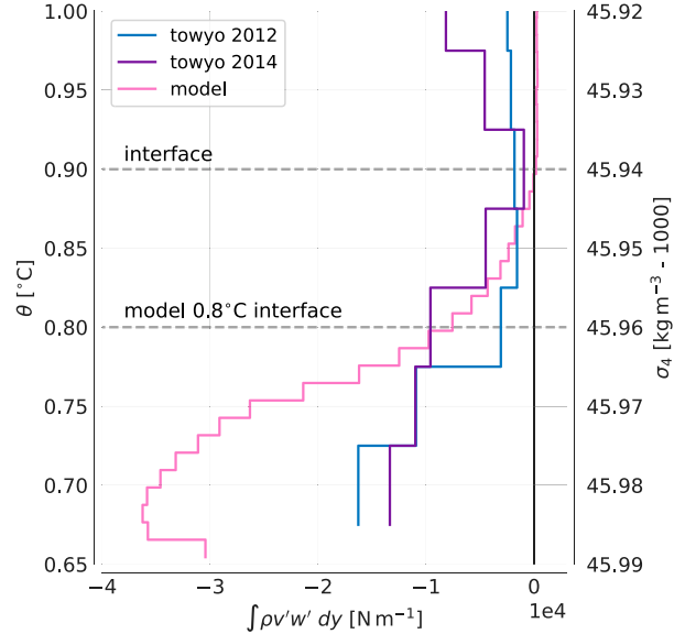
FIG. 14. Vertical flux of horizontal momentum integrated horizontally along isopycnals (for tow-yo observations) and isotherms (for model output) between kilometers 0 and 17. The dashed line indicates the upper interface of the dense bottom layer at \sigma_4 = 45.94 \text{ kg m}^{-3} in the observations and, correspondingly in the temperature-only stratified model, \theta = 0.8^\circ or \theta = 0.9^\circ\text{C} .
