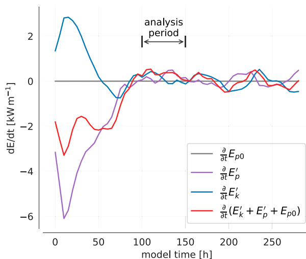
FIG. 7. Rate of change of model perturbation potential energy E_{p0} = 1/2\rho_0 g \eta^2 (gray), baroclinic potential energy E'_p (purple), and baroclinic kinetic energy E'_k (blue) and their sum (red) within a domain centered on the region of interest from kilometers -10 to 30 and bounded in the vertical by the 0.9^\circ\text{C} isotherm. Baroclinic potential and kinetic energy change rapidly during model spinup and stabilize after about 100 h. Model data are analyzed for the period 100–150 h after model start as indicated on the plot. At later times, waves reflected off the model boundaries lead to a less stable flow situation.
