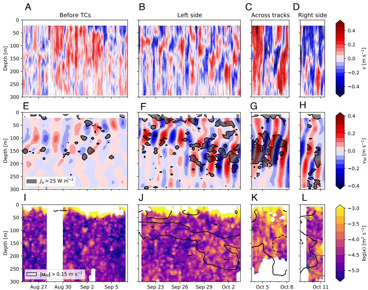
Fig. 2. Upper ocean conditions before and after the passage of three major TCs. Color shading shows (A–D) observed velocities v , their (E–H) bandpass-filtered component v_{NI} , and associated (I–L) 12-h averages of \kappa . Gray hatching in (E–H) outlines areas where 8-h averages of J_q are greater than 25 \text{ W m}^{-2} . Black contours in (I–L) outline areas where \|\mathbf{u}_{NI}\| is greater than (solid) 0.15 and (dashed) 0.3 \text{ m s}^{-1} . Each column represents one of the periods whose temporal averages are shown in Fig. 1.
