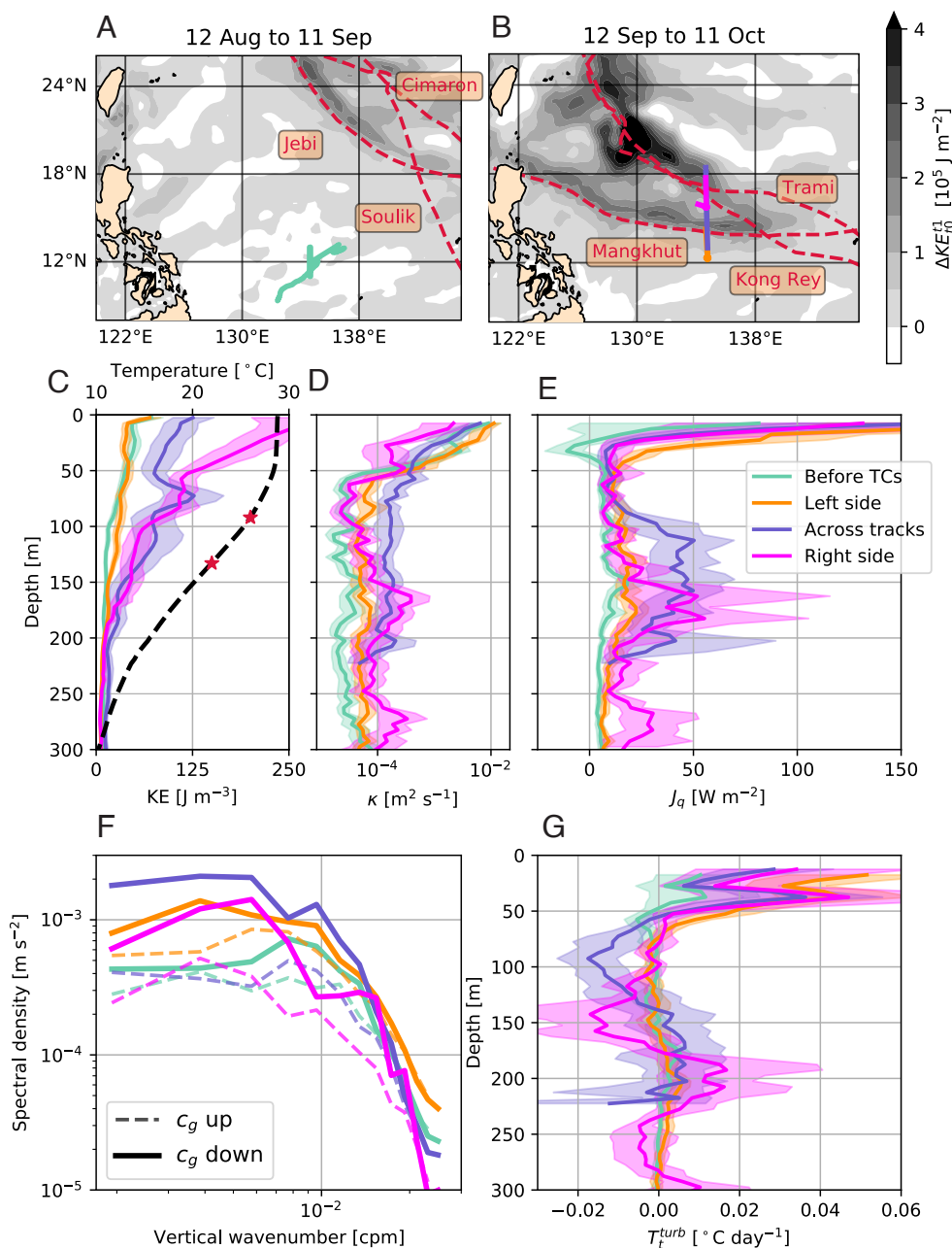
Fig. 1. Ocean effects of wind forcing by TCs. (A and B) \Delta KE integrated over the periods noted in 2018. Mean vertical profiles and 95% confidence intervals of (C) KE , (D) \kappa , and (E) J_q for each of the four periods defined in Fig. 2. (C) shows the mean T(z) across all periods (dashed black line, upper axis), while red stars mark the 22 and 26°C isotherms. (F) vertical wavenumber spectra of shear are shown in dashed and solid lines for rotation associated with upward- and downward-propagating internal wave energy, respectively. (G) T_t^{turb} computed from the convergence of smoothed profiles of J_q in (E).
