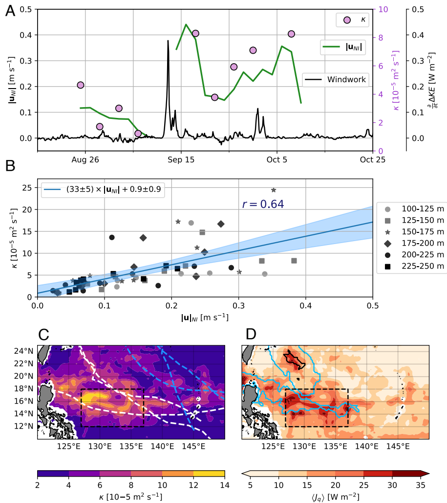
Fig. 4. NIW activity, its relation to \kappa , and regional effects. (A) 4-d averages of |u_{NI}| (green line) and \kappa (pink circles) observed between 125 and 150 m. Windwork \frac{\partial}{\partial t} \Delta KE at the mooring site is shown in black. (B) Linear fit on 4-d averages of observed |u_{NI}| and \kappa at different depths ( r = 0.64 ). Mean values of (C) \kappa and (D) J_q at the 22°C isotherm between September 12 and October 11 inferred from |u_{NI}|^{\text{HYCOM}} . The blue contour in (D) shows areas of SST cooling > 1^\circ\text{C} induced by TCs, while the black contour denotes an area where z_L was deeper than the 22°C isotherm. The dashed box is the area whose averages are described in the main text.
