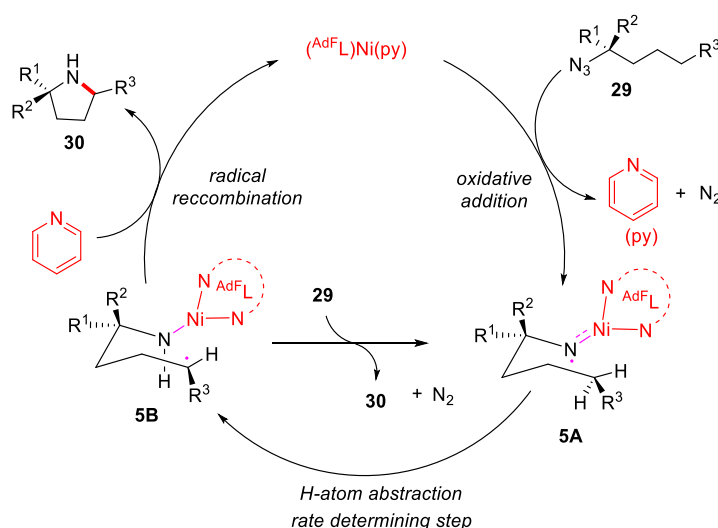
Scheme 11. (a) Dipyrryn-supported nickel catalyst [(\text{AdFL})\text{Ni}(\text{py})] -catalyzed intramolecular C–H bond amination of aliphatic azides; (b) Proposed mechanism.
