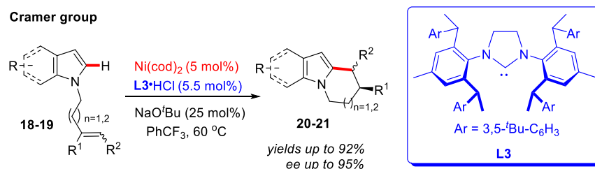
Scheme 8. [M8][k9] Ni(cod) 2 -catalyzed enantioselective C–H functionalization of N -alkenyl-substituted indoles and pyrroles.
