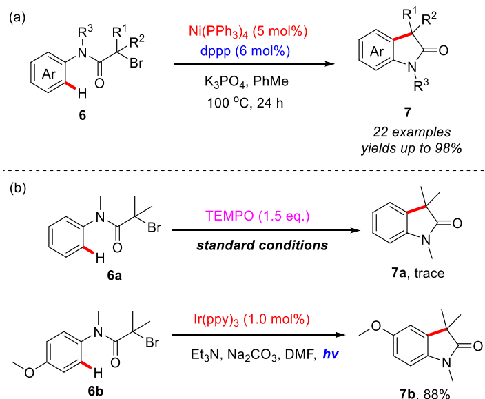
Scheme 3. [M6] (a) \text{Ni(PPh}_3)_4 -catalyzed intramolecular \text{C(sp}^2\text{)-H} alkylation utilizing alkyl-Br bonds for the synthesis of indolones; (b) Radical trapping and visible photocatalysis experiments.
