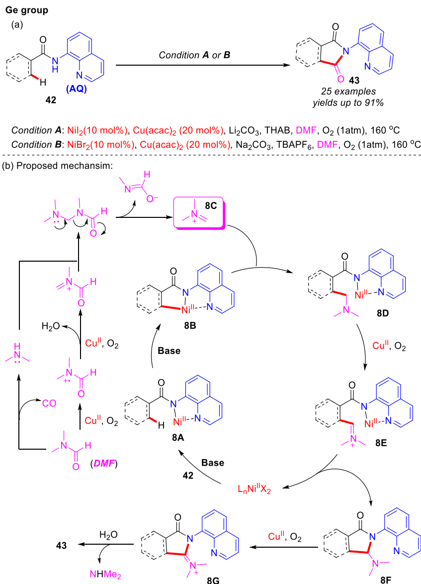
Scheme 16. (a) Ni/Cu co-catalyzed 8-aminoquinoline (8-AQ)-assisted direct C–H carbonylation of amides by using DMF as the CO source under \text{O}_2 atmosphere; (b) Proposed mechanism.
