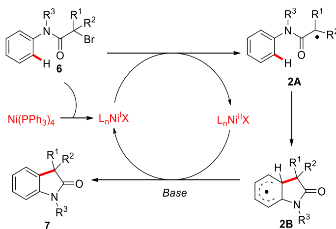
Scheme 4. [M7] Proposed mechanism of \text{Ni(PPh}_3)_4 -catalyzed intramolecular \text{C(sp}^2\text{)-H} alkylation utilizing alkyl-Br bonds.
