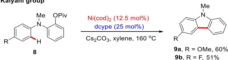
Scheme 5. \text{Ni(cod)}_2 -catalyzed intramolecular C-H arylation of aryl pivalates.
