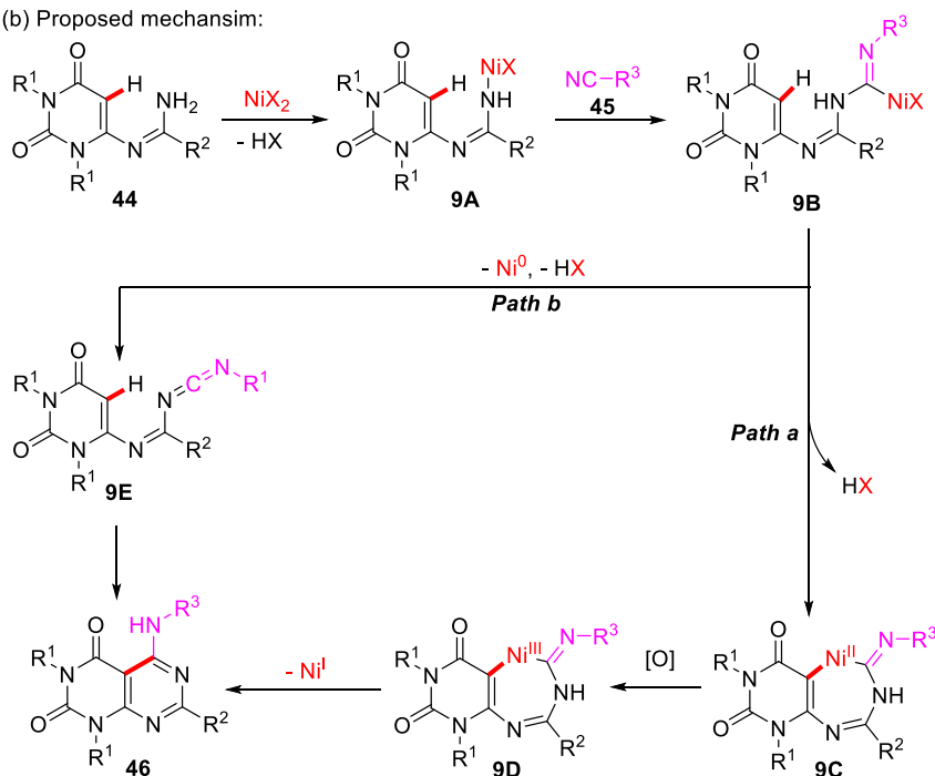
Scheme 17. [M10] (a) Ni(II)-catalyzed oxidative isocyanide insertion/C–H amination reaction; (b) Proposed mechanism.
