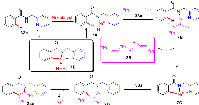
Scheme 13. (a) Ni(cod) 2 -catalyzed directing-group-assisted ortho -C–H functionalization of aromatic amides with alkynes; (b) Proposed mechanism.
