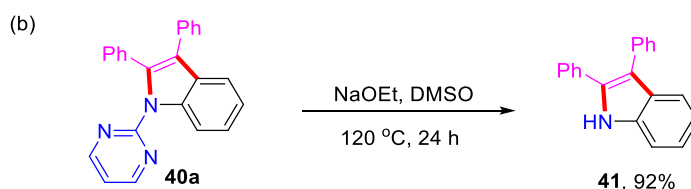
Scheme 15. (a) Ni(cod) 2 -catalyzed C–H oxidative annulation of N -arylpyrimidin-2-amines with symmetrical alkynes; (b) Removal experiment of 2-pyrimidyl group.
