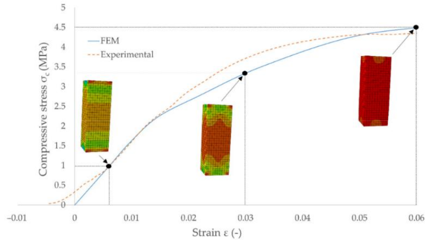
Figure 6 Comparison of FEM model output versus experimental result for tangential compressive stress in 8.74% moisture content pine wood. Source: Wargula et al. [20]; MDPI | reuse permission CC BY.
