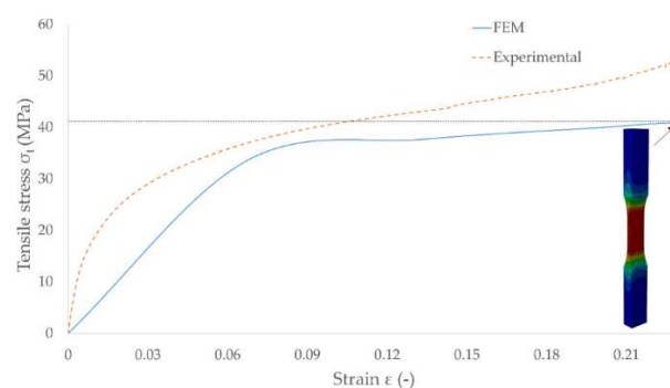
Figure 1 Comparison of FEM model output versus experimental result for longitudinal tensile stress in 19.9% moisture content pine wood. Source: Wargula et al. [20]; MDPI | reuse permission CC BY.
