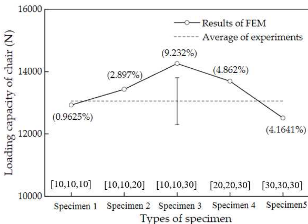
Figure 11 FEM versus experimental outcomes of loading capacities (errors in parentheses) of chair modeled using elastic constants obtained from different specimen configurations. Configurations in square brackets [width, length, height]. Source: Adapted from Hu et al. [44]; MDPI | reuse permission CC BY.
