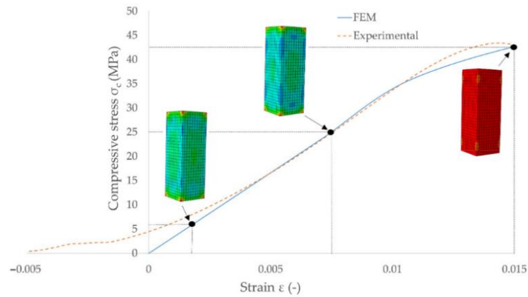
Figure 3 Comparison of FEM model output versus experimental result for longitudinal compressive stress in 19.9% moisture content pine wood. Source: Wargula et al. [20]; MDPI | reuse permission CC BY.
