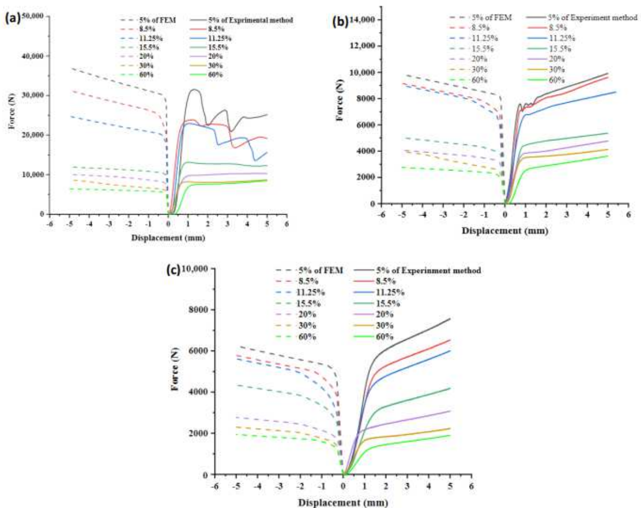
Figure 13 Comparison of FEM and experimental compressive force versus displacement curves at varied moisture loading percentages in beech wood tested at (a) longitudinal, (b) radial, and (c) tangential grain orientations. Source: Fu et al. [66]; MDPI | reuse permission CC BY.
