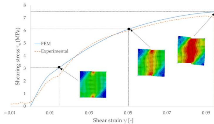
Figure 7 Comparison of FEM model output versus experimental result for longitudinal-radial plane shear stress in 19.9% moisture content pine wood. Source: Wargula et al. [20]; MDPI | reuse permission CC BY.
