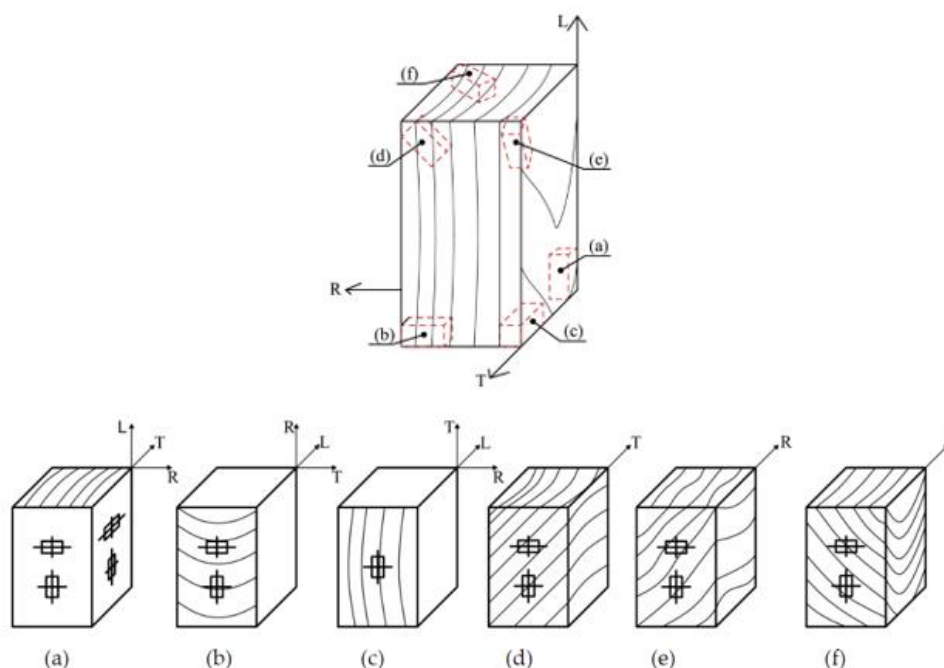
Figure 9 Specimen cutting procedure (top) and configurations (down) for determination of orthotropic elastic constants (i.e., for grain orientations in longitudinal (L), radial (R), and tangential (T) directions). Source: Hu et al. [44]; MDPI | reuse permission CC BY.
