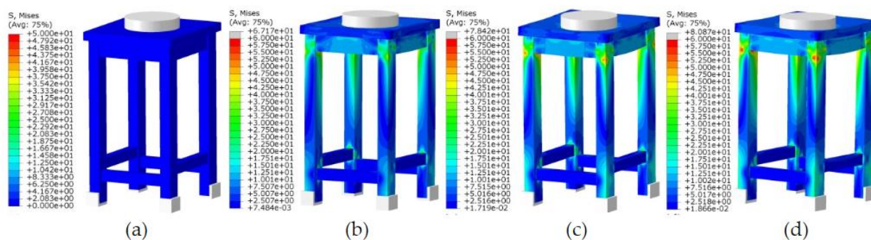
Figure 10 FEA results of stress distribution states in chair model at (a) zero, (b) 1 mm, (c) 2 mm, and (d) 3 mm displacements. Source: Hu et al. [44]; MDPI | reuse permission CC BY.
