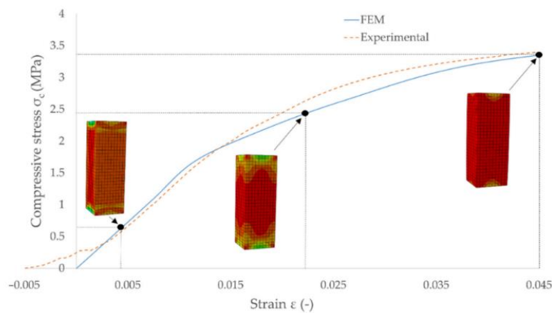
Figure 4 Comparison of FEM model output versus experimental result for tangential compressive stress in 19.9% moisture content pine wood. Source: Wargula et al. [20]; MDPI | reuse permission CC BY.
