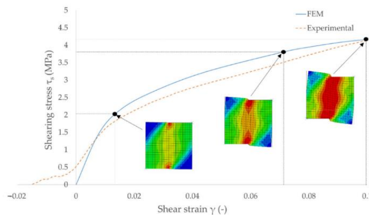
Figure 8 Comparison of FEM model output versus experimental result for radial-tangential plane shear stress in 8.74% moisture content pine wood. Source: Wargula et al. [20]; MDPI | reuse permission CC BY.
