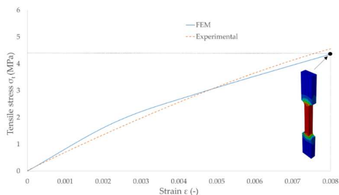
Figure 2 Comparison of FEM model output versus experimental result for radial tensile stress in 8.74% moisture content pine wood. Source: Wargula et al. [20]; MDPI | reuse permission CC BY.
