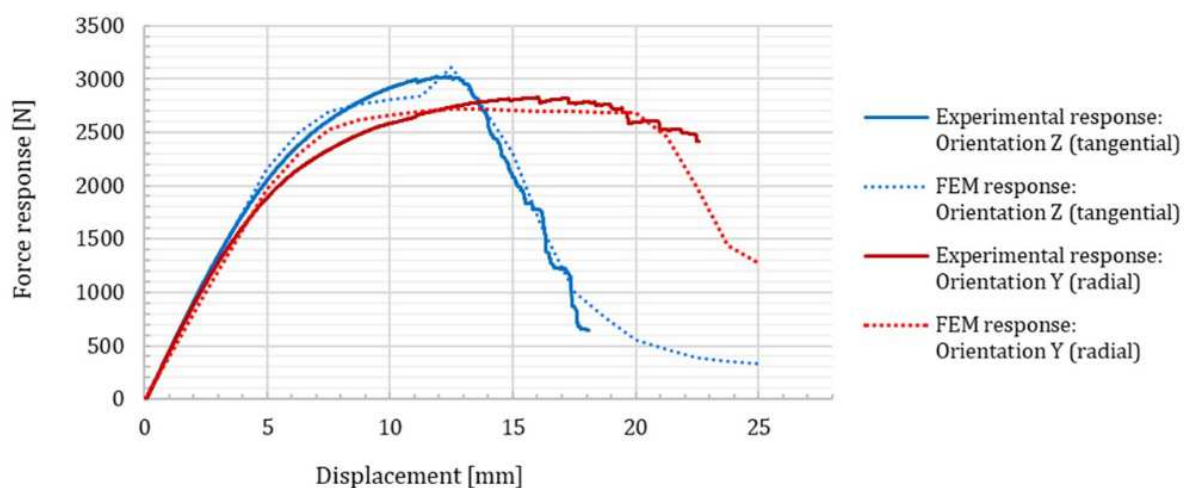
Figure 12 Comparison of FEM versus experimental force-displacement curves obtained from the three-point bending test of spruce wood. Source: Fajdiga et al. [42]; MDPI | reuse permission CC BY.
