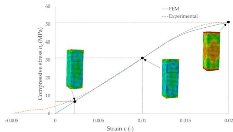
Figure 5 Comparison of FEM model output versus experimental result for longitudinal compressive stress in 8.74% moisture content pine wood. Source: Wargula et al. [20]; MDPI | reuse permission CC BY.
