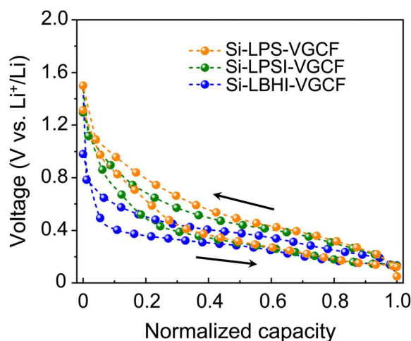
Fig. 3 GITT-derived equilibrium potential curves of Si anodes for the second cycle. The capacity of three anodes was normalized for ease of comparison. The mass ratio of micro-sized Si, SE, and VGCF is 4 : 6 : 1. The current value is 210 \text{mA g}_{\text{Si}}^{-1} . The cut-off voltage range is 0.05–1.5 V vs. \text{Li}^+/\text{Li} .
