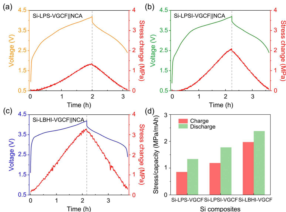
Fig. 6 Pressure change during the first charge and discharge of Si||NCA full cells with (a) Si-LPS-VGCF, (b) Si-LPSI-VGCF, and (c) Si-LBHI-VGCF anodes. (d) Stress change is normalized by the corresponding capacity of the full cells shown in (a), (b), and (c). These full cells were prepared and tested at the same conditions as the full cells shown in Fig. 5.
