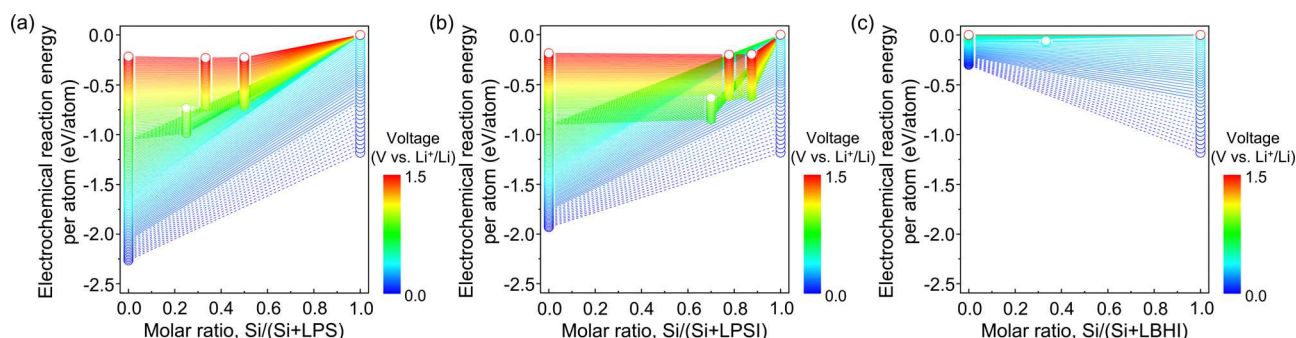
Fig. 1 Calculated electrochemical reaction energies between Si and (a) LPS, (b) LPSI, and (c) LBHI SEs. At a molar fraction of 0, the reaction energy for the electrochemical decomposition of SE itself is reflected; at a molar fraction of 1, only the reaction energy for Si lithiation is calculated. The dashed lines indicate the reaction energy below 0.12 V vs. \text{Li}^+/\text{Li} , where \text{Li}_{21}\text{Si}_5 (at molar fraction of 1) is only available in calculations. The voltage interval used for calculations is 0.01 V vs. \text{Li}^+/\text{Li} . The color bar represents a voltage range of 0.0–1.5 V vs. \text{Li}^+/\text{Li} .
