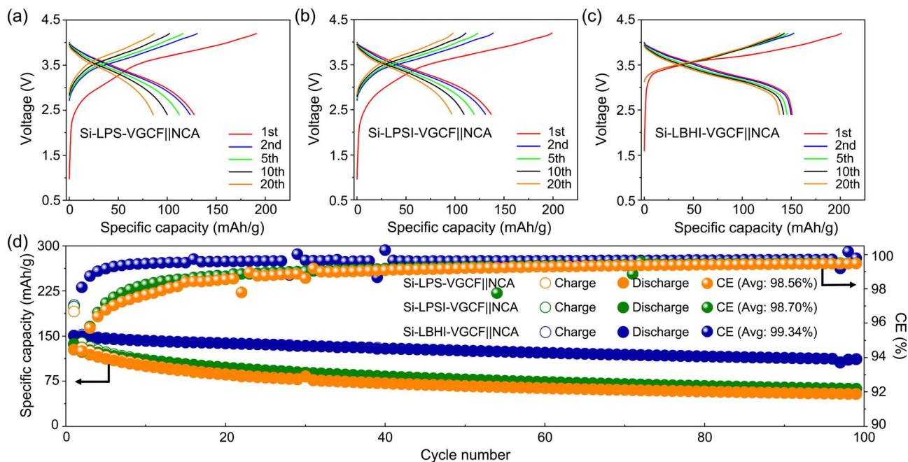
Fig. 5 Electrochemical performance of solid-state Si||NCA full cells. Charge/discharge profiles of solid-state Si||NCA full cells with (a) Si-LPS-VGCF, (b) Si-LPSI-VGCF, and (c) Si-LBHI-VGCF anodes. (d) Cycling performance and CEs of Si||NCA full cells with different anodes. The mass ratio of micro-sized Si, SE, and VGCF is 6 : 4 : 1. The cells were tested at 0.5C (= 0.785 mA) within a voltage range of 2.4–4.2 V at 60 °C. The areal capacity of cathode active materials is 2 mA h cm -2 .
