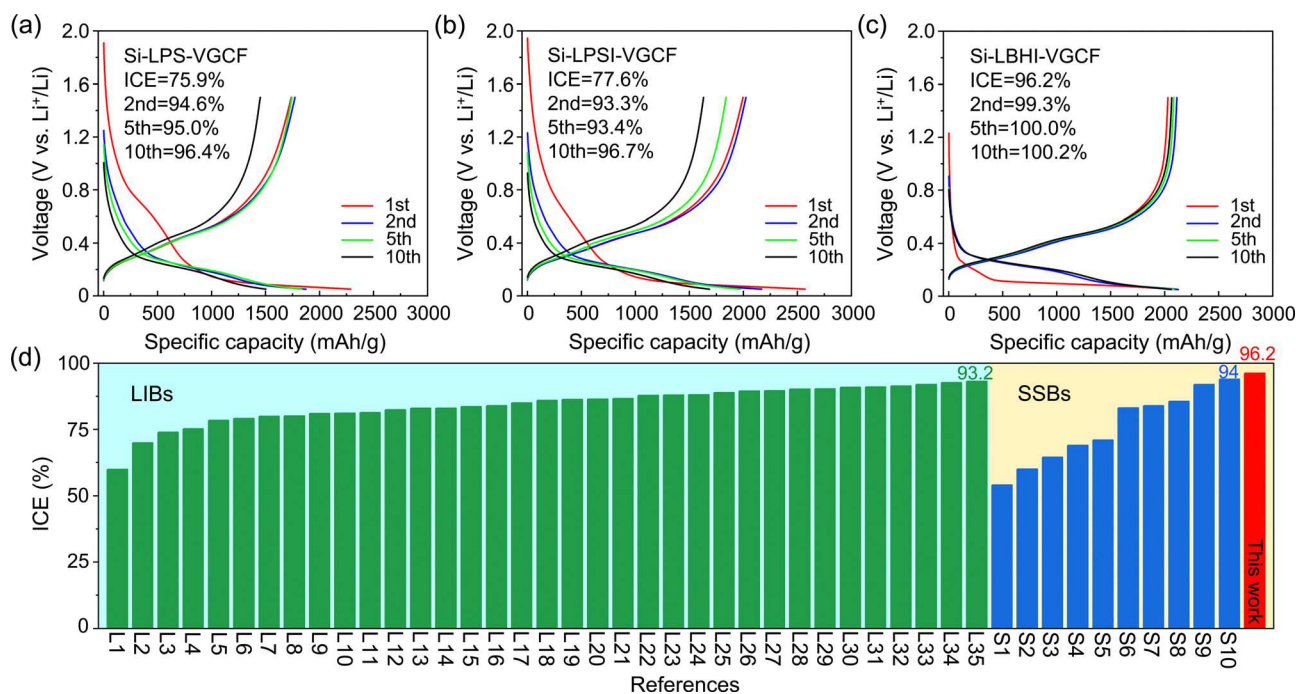
Fig. 2 (a–c) Charge/discharge curves of Si anodes using (a) LPS, (b) LPSI, and (c) LBHI SEs. The anode composites are denoted as Si-LPS-VGCF, Si-LPSI-VGCF, and Si-LBHI-VGCF based on the SE used. The current is 210 \text{ mA g}_{\text{Si}}^{-1} and the voltage range is 0.05–1.5 V vs. \text{Li}^+/\text{Li} (or –0.55–0.9 V vs. Li-In) at 60^\circ\text{C} . The Si composites were prepared by ball milling micro-sized Si, SE, and VGCF in a mass ratio of 6:4:1. (d) Comparison of the ICEs of Si electrodes reported in LIBs and SSBs. The references for the listed ICEs are included in Table S6 (ESI†).
