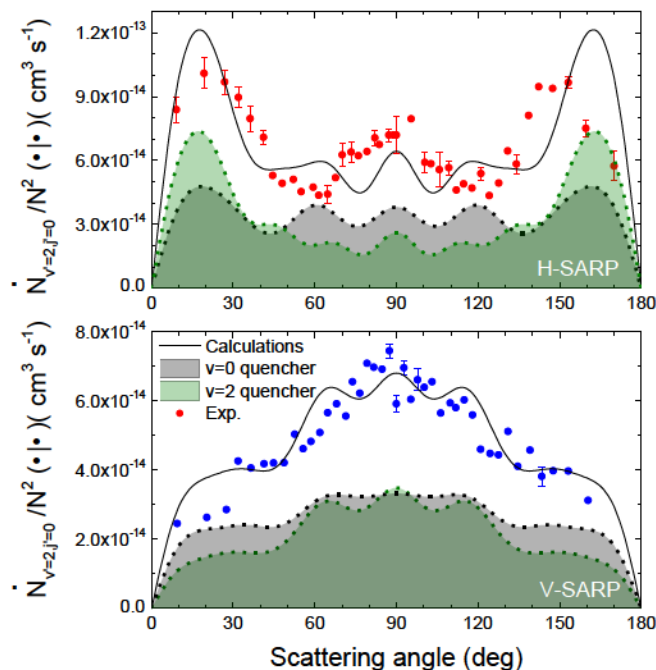
FIG. 4. Velocity-averaged differential rates for D_2(v'=2, j'=0) production normalized by the square of the total density of D_2 (see SI for further details). Results of our calculations are shown in solid curves while experimental results of Zhou et al. [31] are shown in dots. Calculations using a H-SARP (V-SARP) preparation are shown in the top (bottom) panels. Differential rate coefficients were symmetrized as in the experimental work. The contribution of collisions between two D_2 ( v=2 ) molecules is shown in shaded dark green, while that from collisions between one D_2 ( v=2 ) and one D_2 ( v=0 ) is shown in shaded gray and black dashed line.
