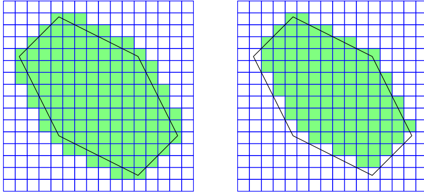
FIGURE 2. Construction in Theorem 3.1 for scaling parameter n = 10 .
