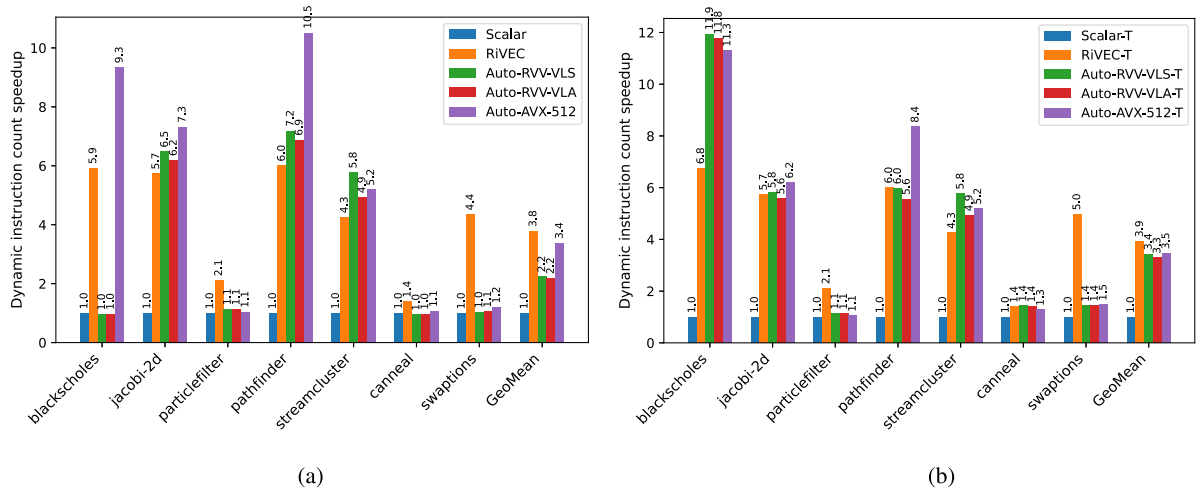
FIGURE 1. Dynamic instruction count speedup over the scalar version using a vector length of 8. Transformations for the auto-vector configurations are based on Table 2, whereas the serial and RlVec versions are transformed to skip math functions only. (a) Unmodified benchmarks. (b) Transformed benchmarks (labeled as -T ).
