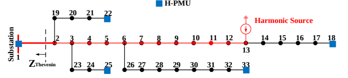
Fig. 1. An example distribution feeder with one harmonic source. In practice, the harmonic current almost entirely flows through the substation.
