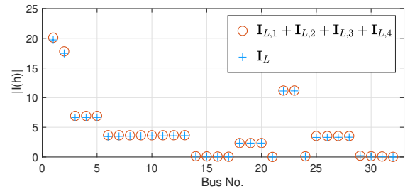
Fig. 9. An illustrative example to validate the superposition theorem among the harmonic state variables. There are four harmonic sources on the network.
