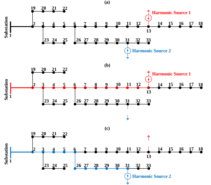
Fig. 2. An example distribution feeder with multiple harmonic source. In practice, the harmonic current almost entirely flows through the substation.
