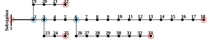
Fig. 3. Three groups of buses on a radial feeder: 1) the buses that are circled in red, 2) the buses that are circled in blue, and 3) the rest of the buses.
