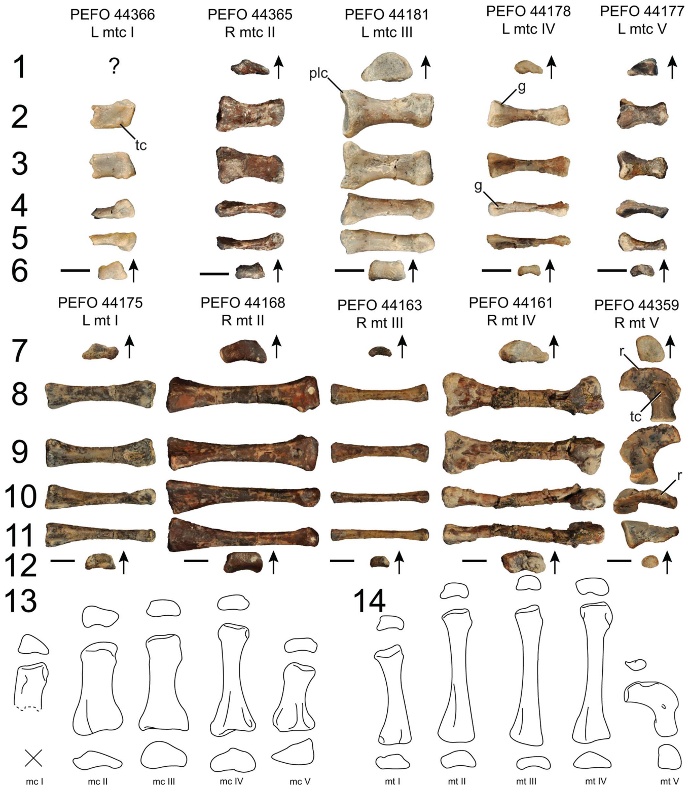
Figure 14. Puercosuchus traverorum n. gen. n. sp. in proximal (1, 7), dorsal (2, 8), ventral (3, 9), lateral (4, 10), medial (5, 11), and distal (6, 12) views. (1–6) Metacarpals; (7–12) metatarsals; reconstructions of right metacarpals (13) and right metatarsals (14) are shown in proximal, dorsal, and distal views. Arrows point in dorsal direction. g = groove; mtc = metacarpal; mt = metatarsal; plc = posterolateral corner; r = ridge; tc = tubercle. Scale bars = 1 cm.
