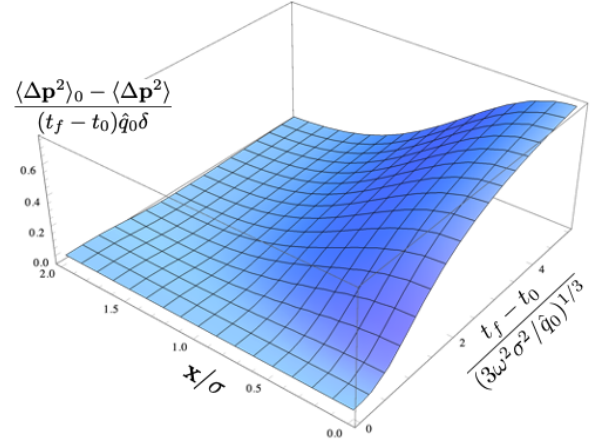
FIG. 4. The reduction of scaled momentum broadening (\langle \Delta \mathbf{p}^2 \rangle_0 - \langle \Delta \mathbf{p}^2 \rangle) / (t_f - t_0) \hat{q}_0 \delta as a function of the scaled transverse position \mathbf{x}/\sigma and propagation time (t_f - t_0) / (3\omega^2 \sigma^2 / \hat{q}_0)^{1/3} .
