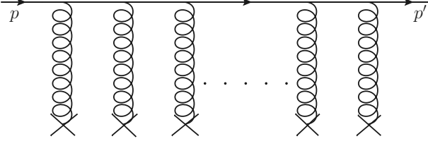
FIG. 1. Illustration of the eikonal propagation of a quark with initial momentum p and final momentum p' in the medium, where the 'cross' donates medium field.
