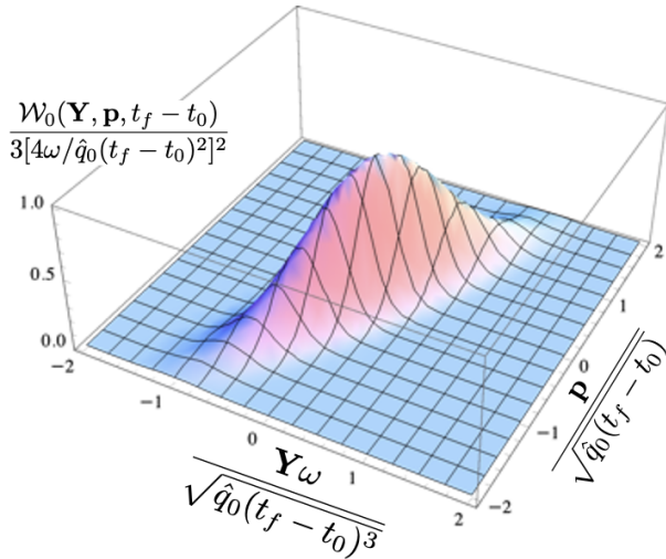
FIG. 2. The scaled Wigner distribution for an initial classical parton in a uniform medium with a constant jet transport coefficient \hat{q}_0 given by Eq. (37) as a function of the transverse momentum and coordinate, both scaled by their respective widths, \sqrt{\hat{q}_0(t_f - t_0)} and \sqrt{\hat{q}_0(t_f - t_0)^3}/\omega .
