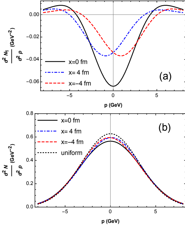
FIG. 3. (a) The first-order correction and (b) the final transverse momentum distribution for initial position x = -4.0 fm (red dashed), 0.0 (black solid), 4.0 (blue dot-dashed) fm, \omega = 5 GeV, t_f - t_0 = 10 fm/c, \hat{q}_0 = 2 GeV 2 /fm, \delta = 0.1 and \sigma = 5 fm in the simple model for an inhomogeneous jet transport coefficient. The dotted line is the distribution in a uniform medium with a constant jet transport coefficient \hat{q}_0 .
