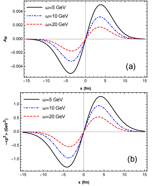
FIG. 5. Transverse momentum asymmetry as a function of the initial transverse position x for t_f - t_0 = 10 fm/c, \hat{q}_0 = 2 \text{GeV}^2/\text{fm} , \delta = 0.1 , \sigma = 5 fm in the simple model.
