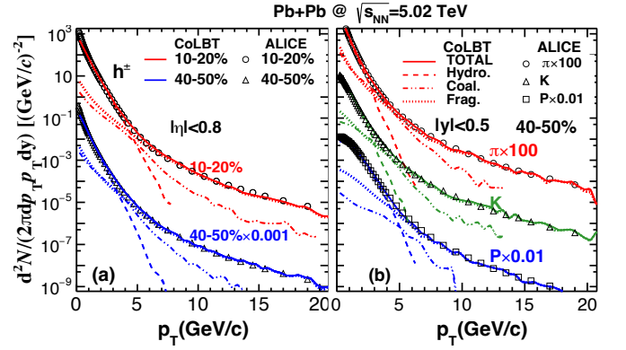
FIG. 2. (Color online) Spectra of (a) charged hadrons (solid) in 10-20% and 40-50% and (b) identified \pi , K and p (solid) in 40-50% Pb+Pb collisions at \sqrt{s_{NN}} = 5.02 TeV and contributions from hydro freeze-out (dashed), parton coalescence (dot-dashed) and fragmentation (dotted) in CoLBT-hydro simulations as compared to ALICE experimental data [111, 112].
