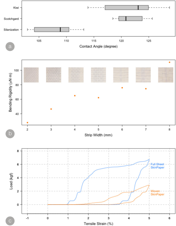
Figure 7: (a) Contact angle measurements of washi paper with three treatments: Silanization with trichlorododecylsilane, the Scotchgard Sun and Water Shield, and the Kiwi Camp Dry spray. (b) Bending rigidity characterization of swatches woven with washi paper at different strip widths. (c) Tensile strength comparison between full sheets and woven hydrophobic washi paper
