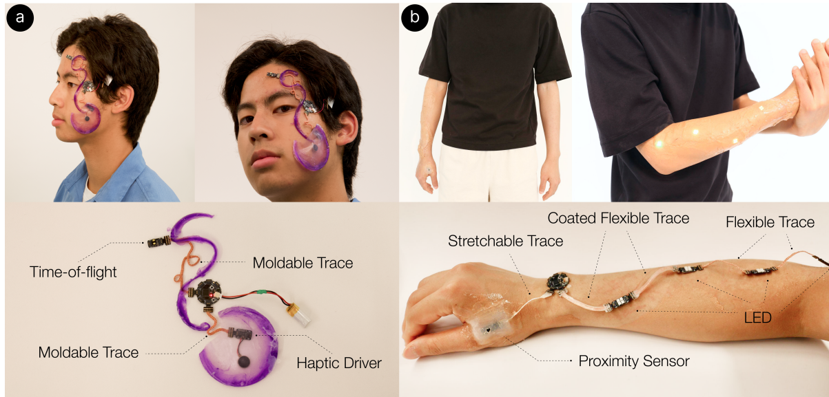
Fig. 13. (a) Victoria's project created a heartbeat on the cheek. She winded moldable trace modules to create intricate patterns paired with silicone prosthetics. The circuit consists of a time-of-flight sensor and a haptic driver. (b) Madison's project hid a proximity alarm on the forearm. She used a skin-tone foundation to camouflage the circuit with a thin layer of prosthetic skin. Four LED modules will light up gradually when the proximity sensor detects an object getting closer.
