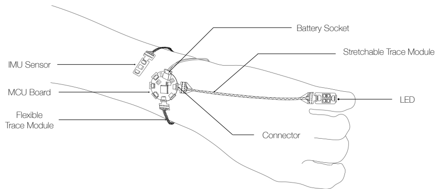
Fig. 2. Example diagram of a SkinLink device. The sensor and actuator modules connect to the microcontroller board via flexible and stretchable trace modules.
