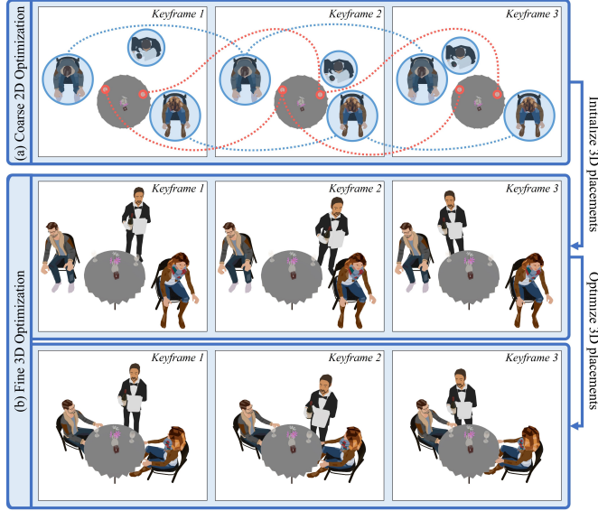
Fig. 6. Our approach instantiates activity snippets in 3D environments by a two-stage optimization. (a) A coarse optimization is performed in 2D space, whose results are projected back to the 3D environment as the initialization for (b) a fine optimization in 3D space.
