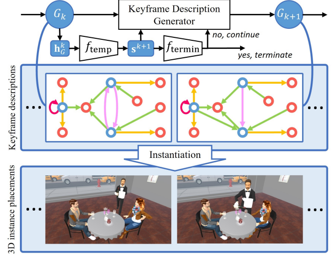
Fig. 2. An overview of our approach. A sequence of keyframe descriptions \{G_k\} is generated by repeatedly producing new keyframe descriptions conditioned on their predecessors, considering spatial-temporal relations. A recurrent temporal function f_{temp} , an LSTM in our implementation, takes in the graph summary h_G^k and outputs a generation signal s^{k+1} . A termination function f_{termin} , an MLP in our implementation, decides whether to end the iterative generation. In the next step, an activity snippet instantiation model, based on an optimization framework, synthesizes placements of instances encoded by the keyframe descriptions as a sequence of 3D scenes.
