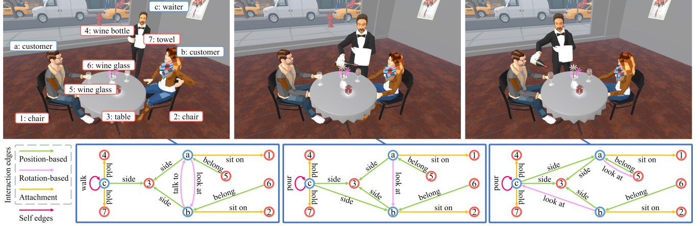
Fig. 3. A generated "serve wine" activity snippet. 3D placements of instances (characters and objects) and their animation assignments are guided by interactions encoded by edges in the keyframe descriptions. Blue nodes denote characters. Red nodes denote objects. Edge colors indicate edge categories.
