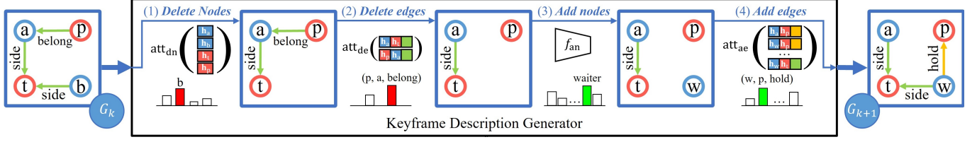
Fig. 4. The workflow of the keyframe description generator. Starting from an input keyframe description G_k , it triggers four modules sequentially to delete nodes, delete edges, add nodes, and add edges, and finally produces the next keyframe description G_{k+1} conditioned on G_k . In this example, nodes a and b refer to two customers. Nodes w , t , and p refer to a waiter, a table, and a plate, respectively.
