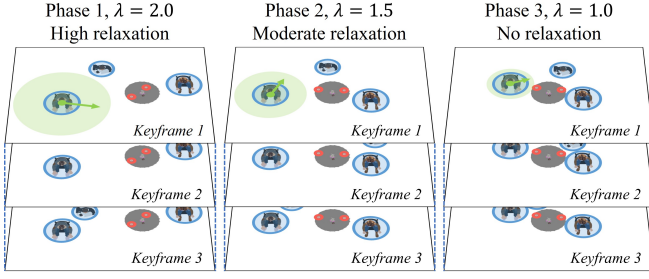
Fig. 7. An example progressive optimization with three sub-optimization phases, where the relaxation factor \lambda drops from 2 to 1. The final placements of instances in all phases are shown in the columns. The larger \lambda is, the more target distances are relaxed in the position-based constraints, and the larger move ranges are allowed as depicted by the green circles. Instances' possible moves during the optimization, as shown by the green arrows, are sampled within the move ranges.
