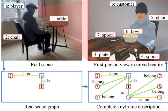
Fig. 13. A "serve food" activity snippet in mixed reality. The real scene graph was used as a partial keyframe description. The generated complete keyframe description, which included both real instances (indicated by rectangular nodes) and augmented virtual instances (indicated by circular nodes), was instantiated and visualized through a mixed reality headset.
