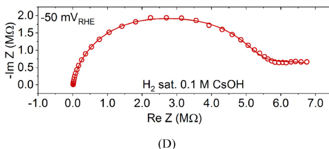
Fig. 4. Typical examples of fitting of the EIS data to the model shown in Fig. 3 for the: (A) LiOH, (B) NaOH, (C) KOH, and (D) CsOH at -0.05 \text{ V} vs RHE. Solid lines represent the fitting, while the points represent the raw data.
