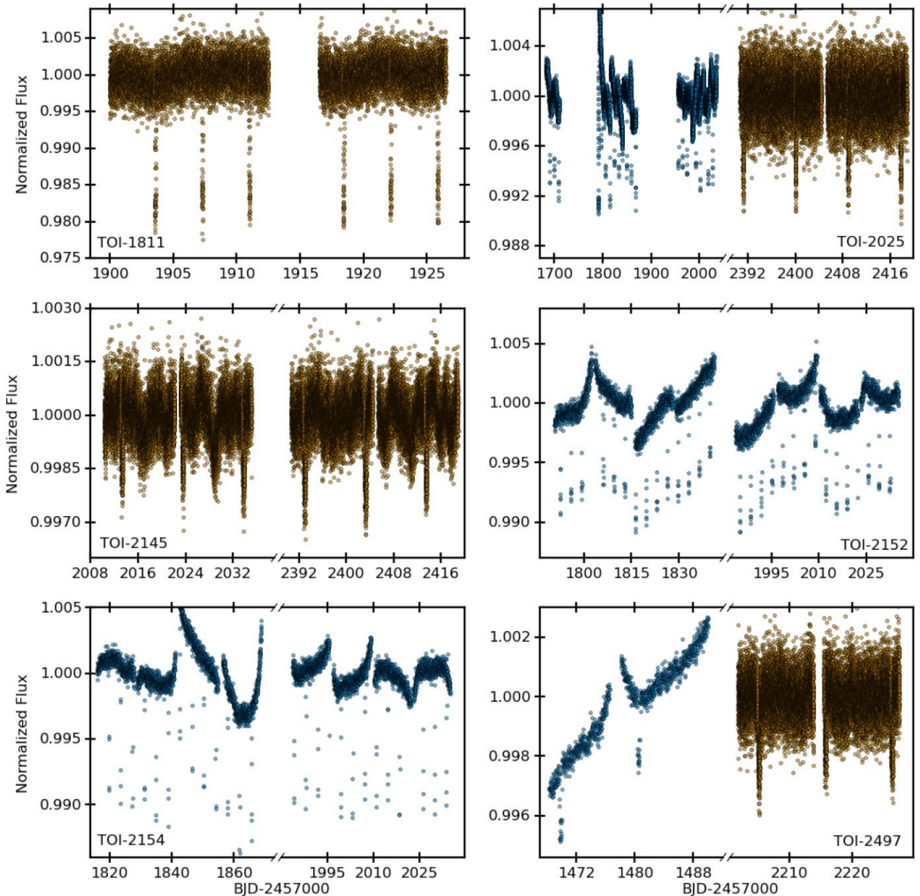
Figure 1. The TESS 30-min light curves extracted using the technique described in Section 2.1 (blue) and 2-min SPOC light curves (orange) for TOI-1811 (top-left), TOI-2025 (top-right), TOI-2145 (middle-left), TOI-2152 (middle-right), TOI-2154 (bottom-left), and TOI-2497 (bottom-right).
